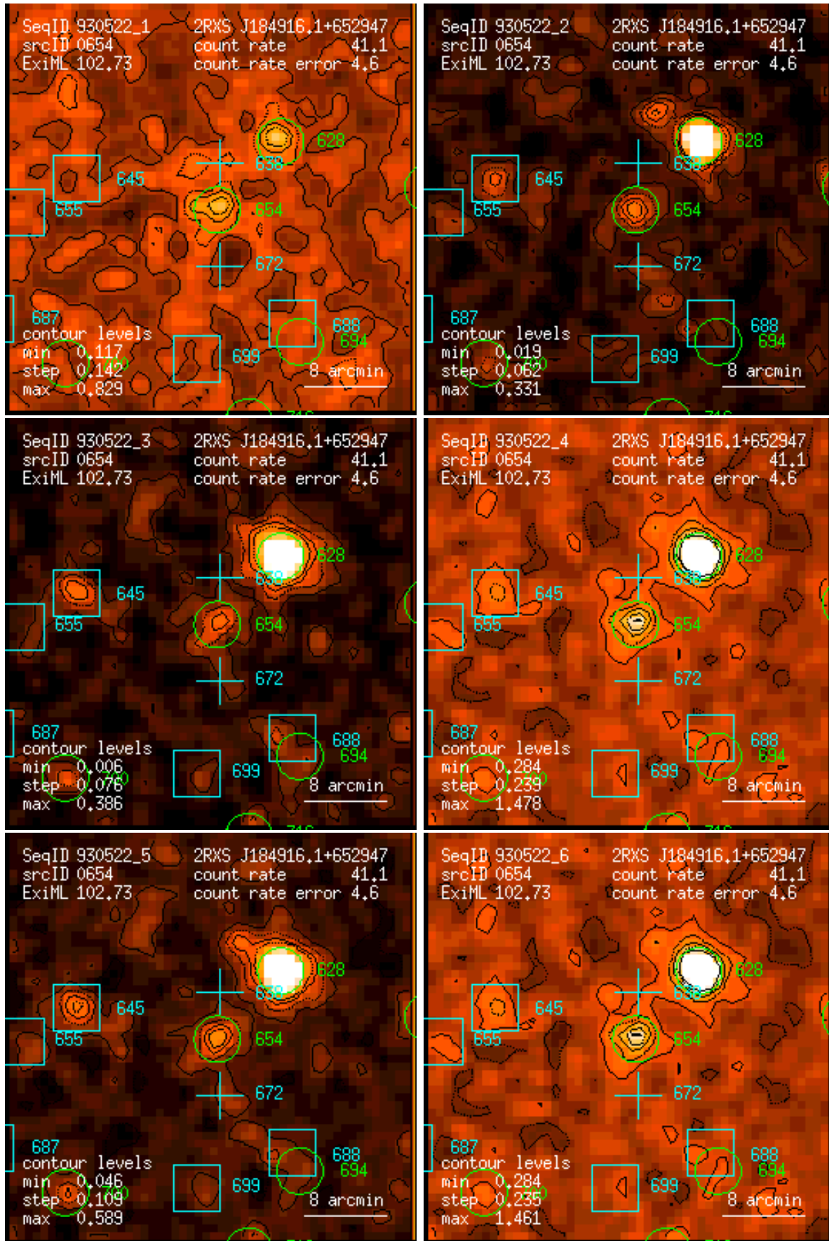
Figure 654: RASS 930522: detection 0654: band rate images, Gaussian filter: (1) PSPC channels 11 – 41, (2) 52 – 90, (3) 91 – 201, (4) 11 – 235, (5) 52 – 201, (6) 11 – 201. Broad band rates in counts/ks. Band rate contour levels in counts/ks/arcmin 2 .
