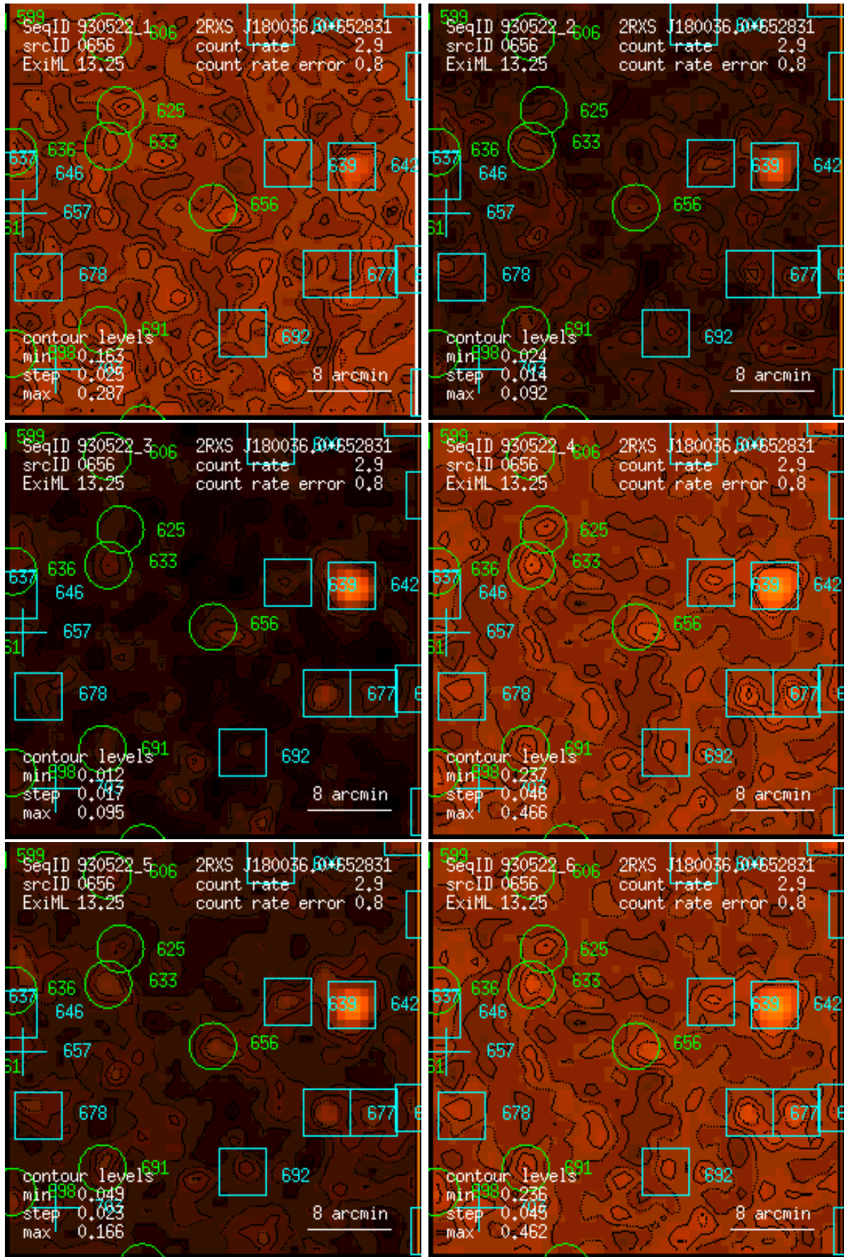
Figure 656: RASS 930522: detection 0656: band rate images, Gaussian filter: (1) PSPC channels 11 – 41, (2) 52 – 90, (3) 91 – 201, (4) 11 – 235, (5) 52 – 201, (6) 11 – 201. Broad band rates in counts/ks. Band rate contour levels in counts/ks/arcmin 2 .
