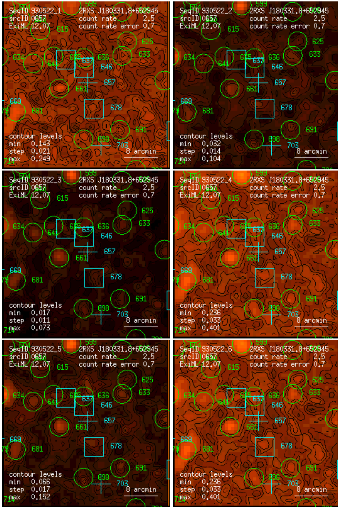
Figure 657: RASS 930522: detection 0657: band rate images, Gaussian filter: (1) PSPC channels 11 – 41, (2) 52 – 90, (3) 91 – 201, (4) 11 – 235, (5) 52 – 201, (6) 11 – 201. Broad band rates in counts/ks. Band rate contour levels in counts/ks/arcmin 2 .
