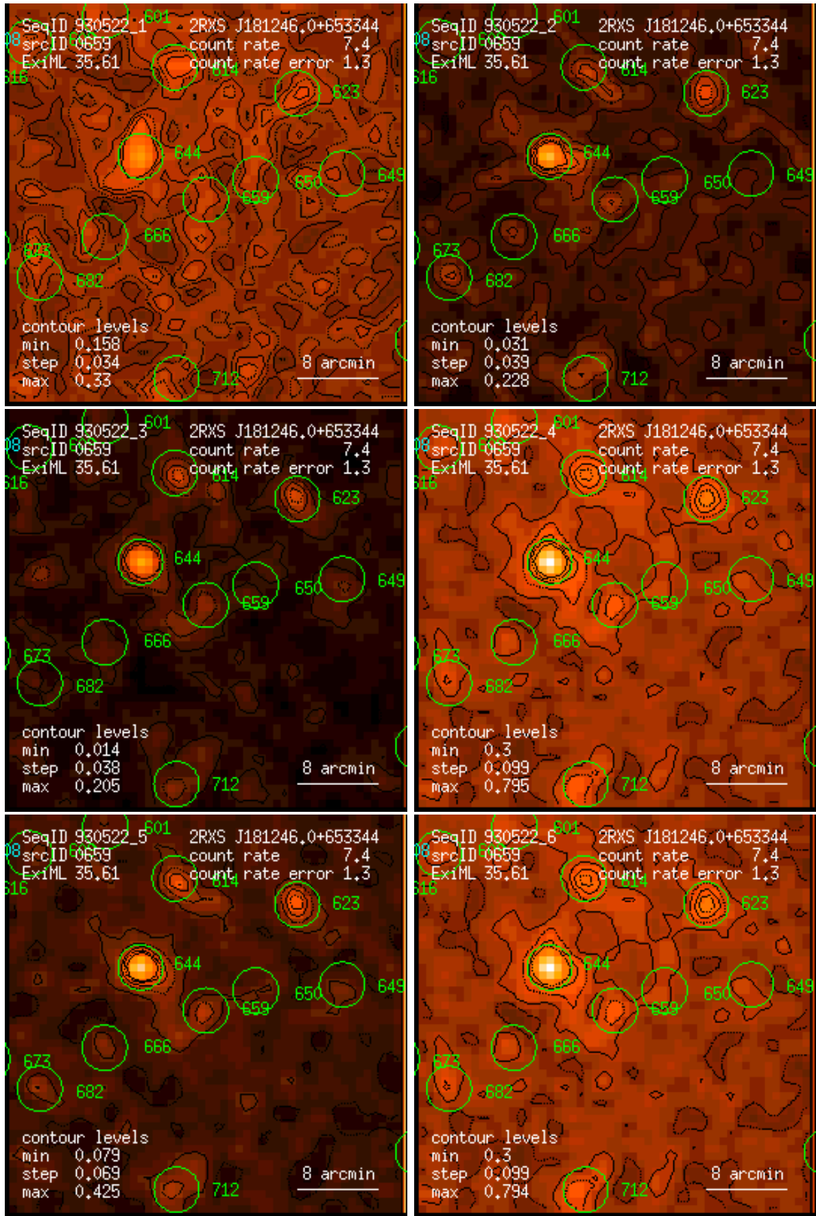
Figure 659: RASS 930522: detection 0659: band rate images, Gaussian filter: (1) PSPC channels 11 – 41, (2) 52 – 90, (3) 91 – 201, (4) 11 – 235, (5) 52 – 201, (6) 11 – 201. Broad band rates in counts/ks. Band rate contour levels in counts/ks/arcmin 2 .
