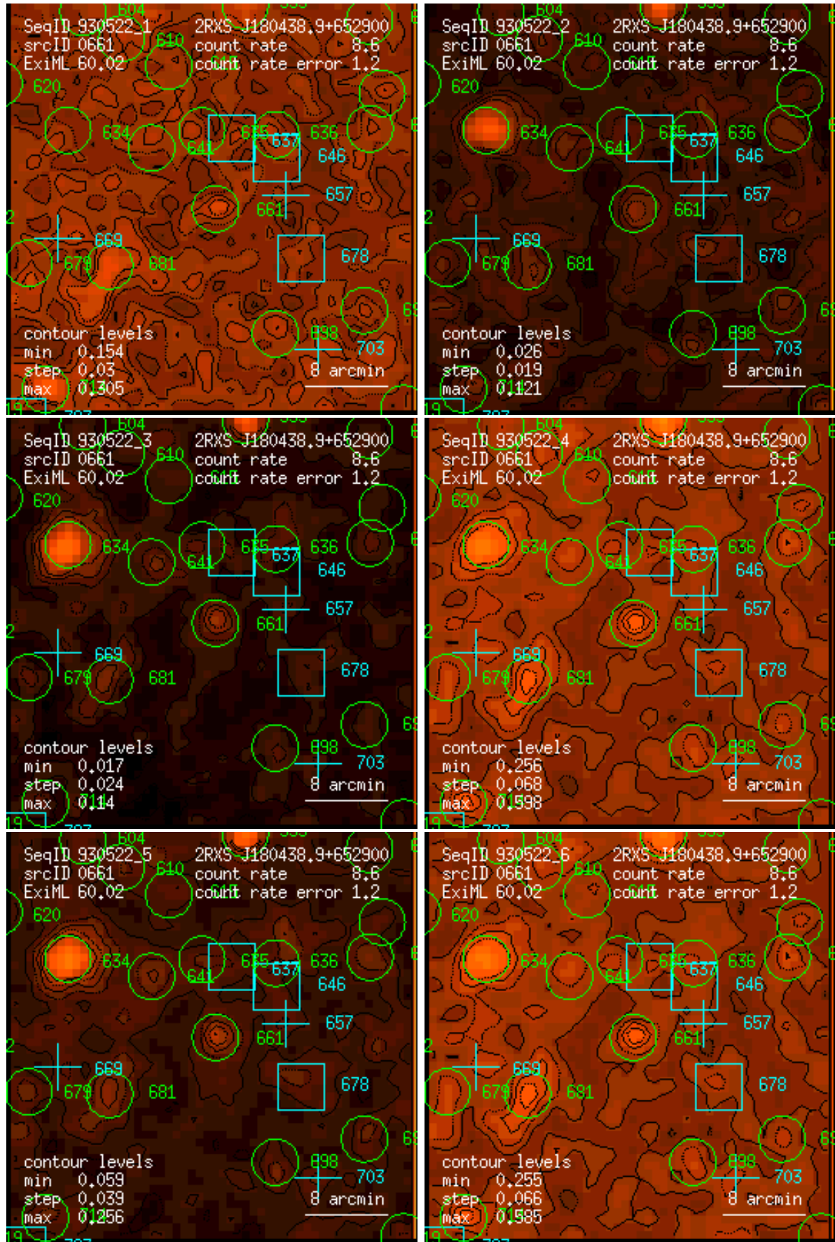
Figure 661: RASS 930522: detection 0661: band rate images, Gaussian filter: (1) PSPC channels 11 – 41, (2) 52 – 90, (3) 91 – 201, (4) 11 – 235, (5) 52 – 201, (6) 11 – 201. Broad band rates in counts/ks. Band rate contour levels in counts/ks/arcmin 2 .
