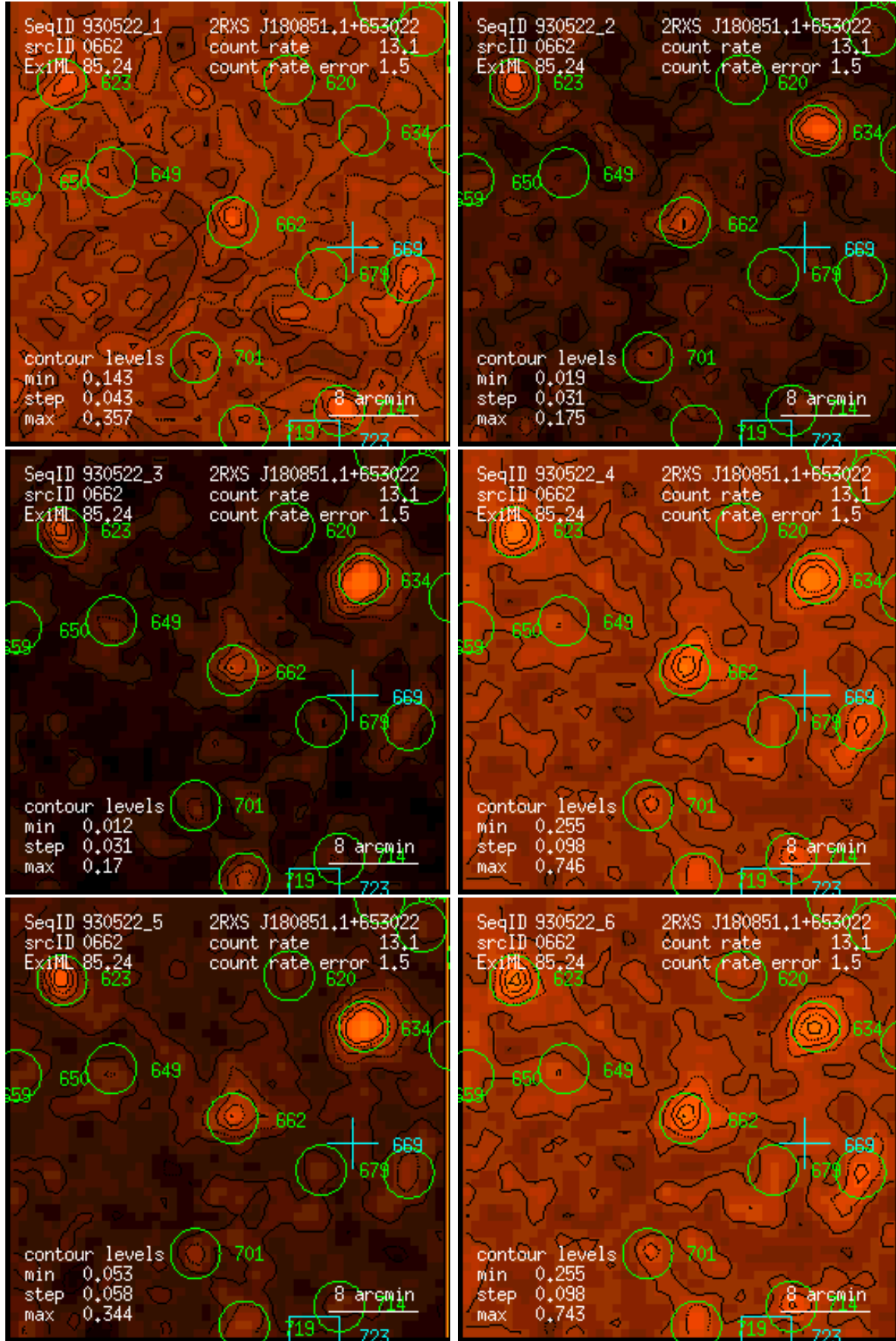
Figure 662: RASS 930522: detection 0662: band rate images, Gaussian filter: (1) PSPC channels 11 – 41, (2) 52 – 90, (3) 91 – 201, (4) 11 – 235, (5) 52 – 201, (6) 11 – 201. Broad band rates in counts/ks. Band rate contour levels in counts/ks/arcmin 2 .
