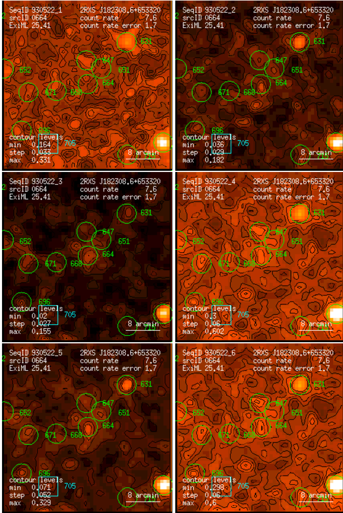
Figure 664: RASS 930522: detection 0664: band rate images, Gaussian filter: (1) PSPC channels 11 – 41, (2) 52 – 90, (3) 91 – 201, (4) 11 – 235, (5) 52 – 201, (6) 11 – 201. Broad band rates in counts/ks. Band rate contour levels in counts/ks/arcmin 2 .
