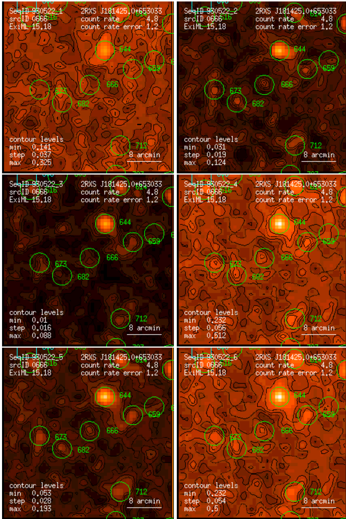
Figure 666: RASS 930522: detection 0666: band rate images, Gaussian filter: (1) PSPC channels 11 – 41, (2) 52 – 90, (3) 91 – 201, (4) 11 – 235, (5) 52 – 201, (6) 11 – 201. Broad band rates in counts/ks. Band rate contour levels in counts/ks/arcmin 2 .
