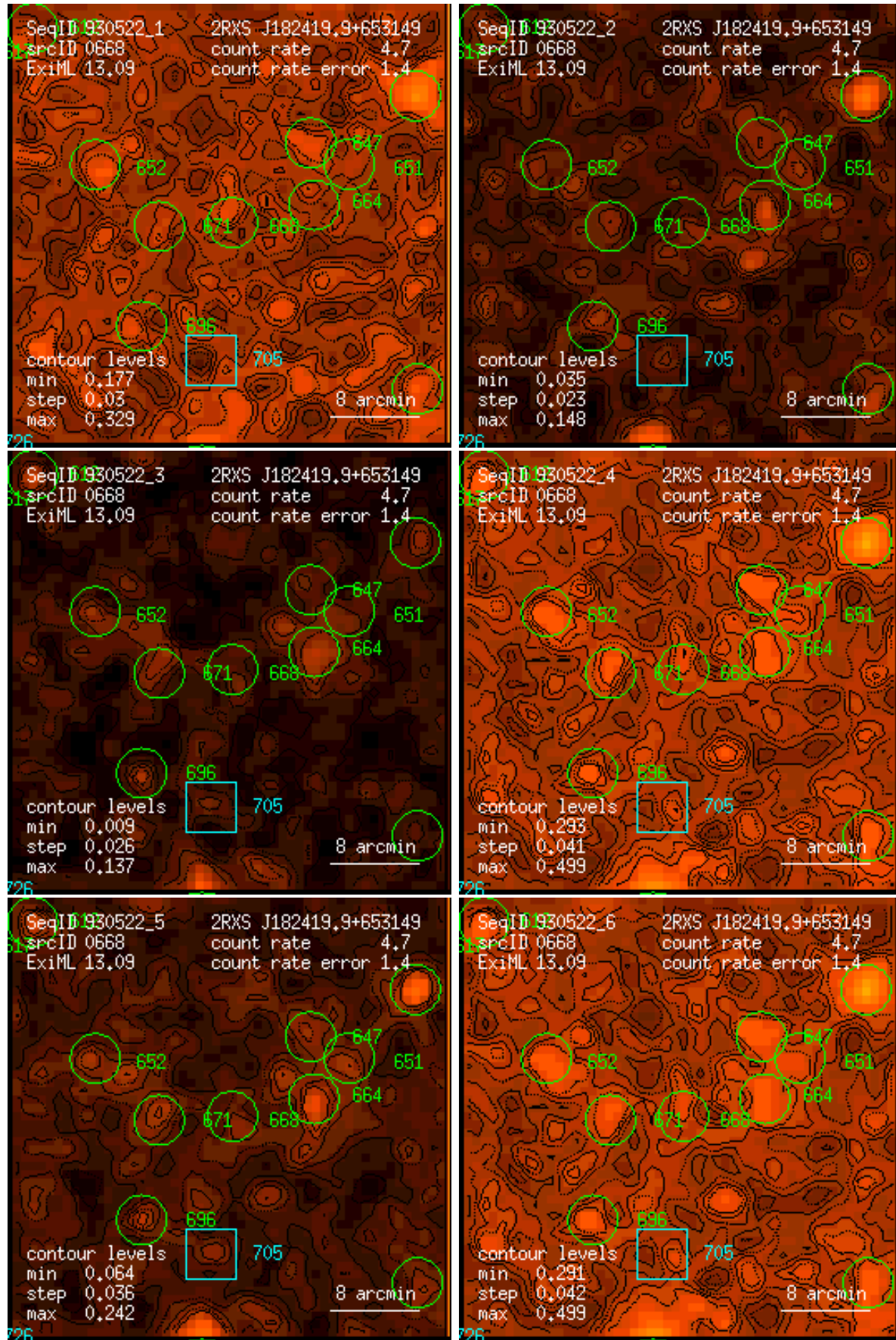
Figure 668: RASS 930522: detection 0668: band rate images, Gaussian filter: (1) PSPC channels 11 – 41, (2) 52 – 90, (3) 91 – 201, (4) 11 – 235, (5) 52 – 201, (6) 11 – 201. Broad band rates in counts/ks. Band rate contour levels in counts/ks/arcmin 2 .
