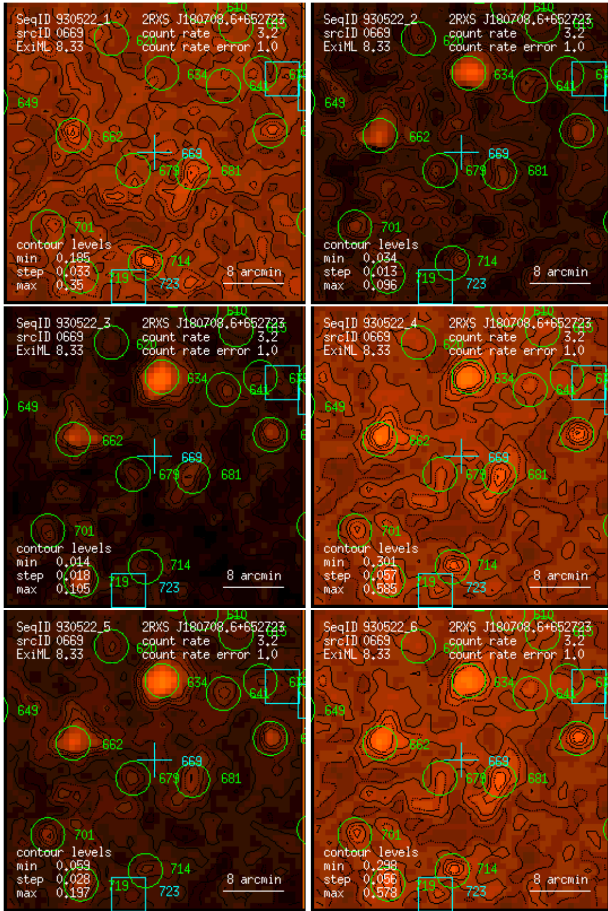
Figure 669: RASS 930522: detection 0669: band rate images, Gaussian filter: (1) PSPC channels 11 – 41, (2) 52 – 90, (3) 91 – 201, (4) 11 – 235, (5) 52 – 201, (6) 11 – 201. Broad band rates in counts/ks. Band rate contour levels in counts/ks/arcmin 2 .
