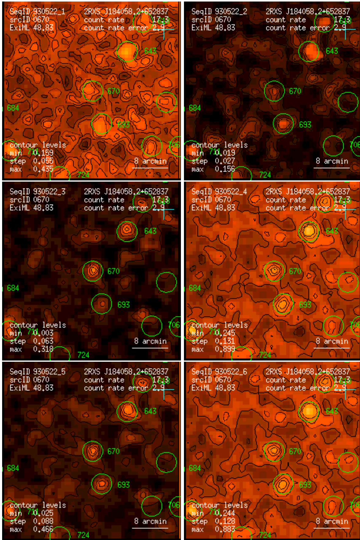
Figure 670: RASS 930522: detection 0670: band rate images, Gaussian filter: (1) PSPC channels 11 – 41, (2) 52 – 90, (3) 91 – 201, (4) 11 – 235, (5) 52 – 201, (6) 11 – 201. Broad band rates in counts/ks. Band rate contour levels in counts/ks/arcmin 2 .
