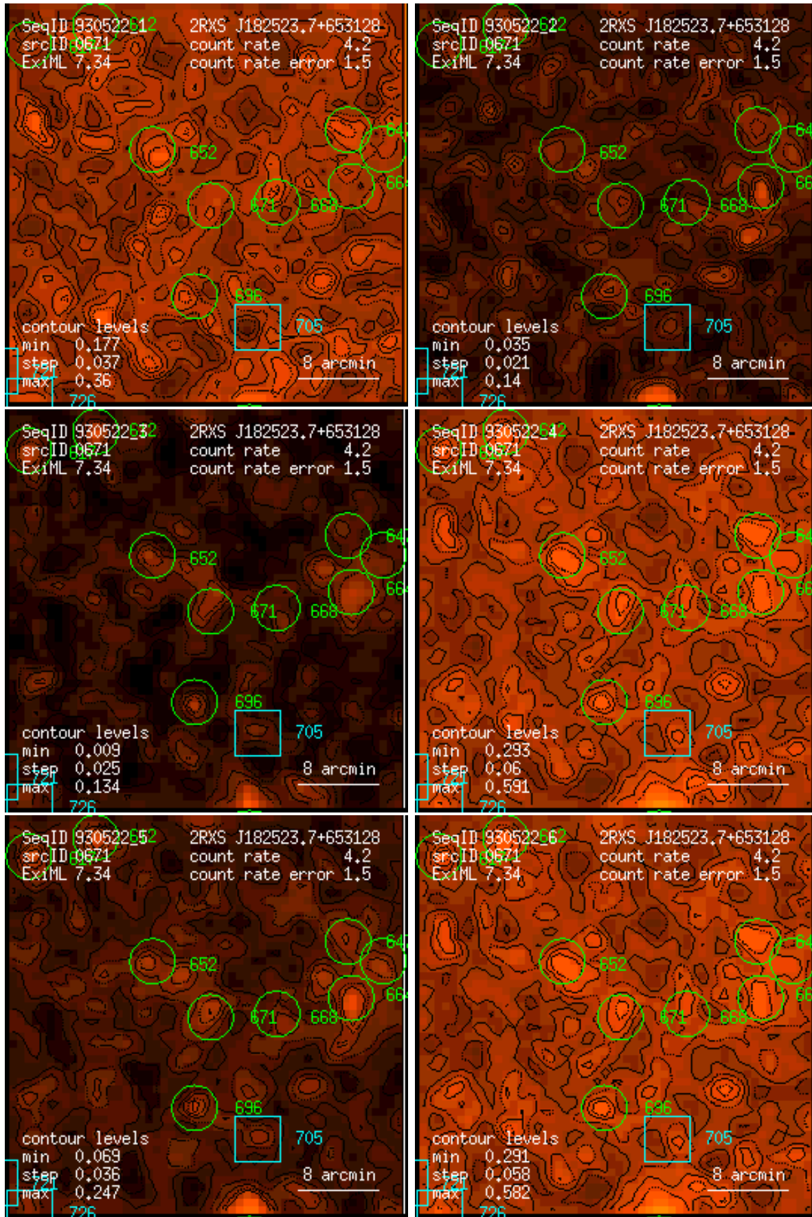
Figure 671: RASS 930522: detection 0671: band rate images, Gaussian filter: (1) PSPC channels 11 – 41, (2) 52 – 90, (3) 91 – 201, (4) 11 – 235, (5) 52 – 201, (6) 11 – 201. Broad band rates in counts/ks. Band rate contour levels in counts/ks/arcmin 2 .
