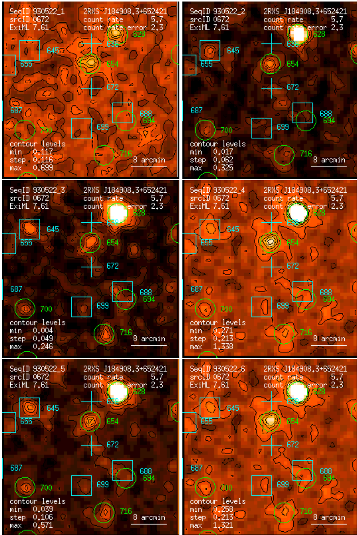
Figure 672: RASS 930522: detection 0672: band rate images, Gaussian filter: (1) PSPC channels 11 – 41, (2) 52 – 90, (3) 91 – 201, (4) 11 – 235, (5) 52 – 201, (6) 11 – 201. Broad band rates in counts/ks. Band rate contour levels in counts/ks/arcmin 2 .
