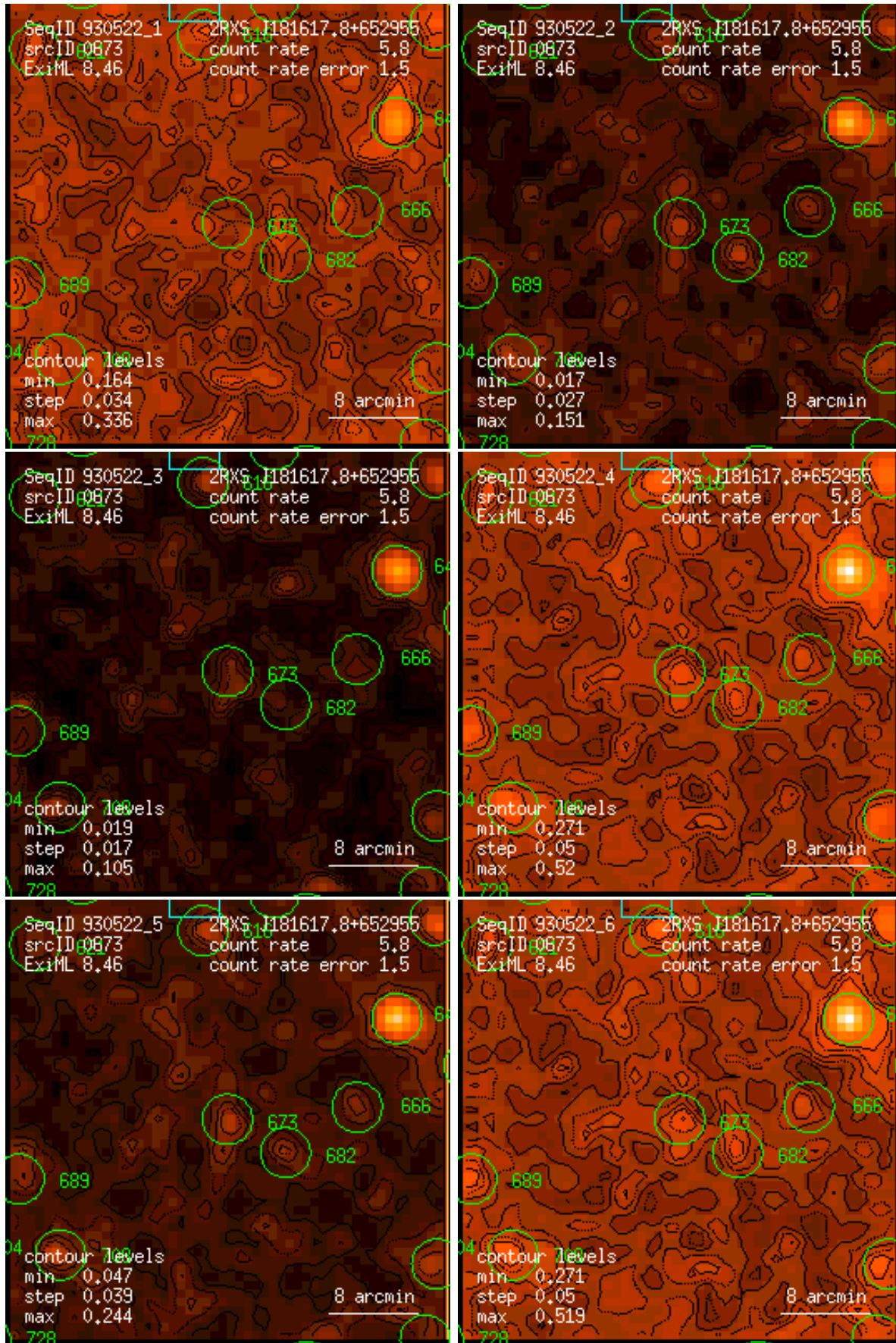
Figure 673: RASS 930522: detection 0673: band rate images, Gaussian filter: (1) PSPC channels 11 – 41, (2) 52 – 90, (3) 91 – 201, (4) 11 – 235, (5) 52 – 201, (6) 11 – 201. Broad band rates in counts/ks. Band rate contour levels in counts/ks/arcmin 2 .
