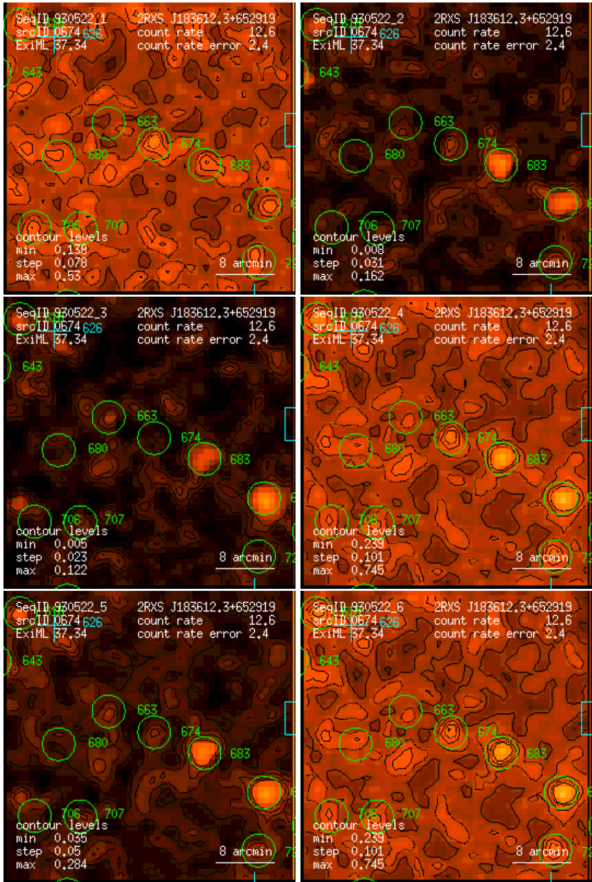
Figure 674: RASS 930522: detection 0674: band rate images, Gaussian filter: (1) PSPC channels 11 – 41, (2) 52 – 90, (3) 91 – 201, (4) 11 – 235, (5) 52 – 201, (6) 11 – 201. Broad band rates in counts/ks. Band rate contour levels in counts/ks/arcmin 2 .
