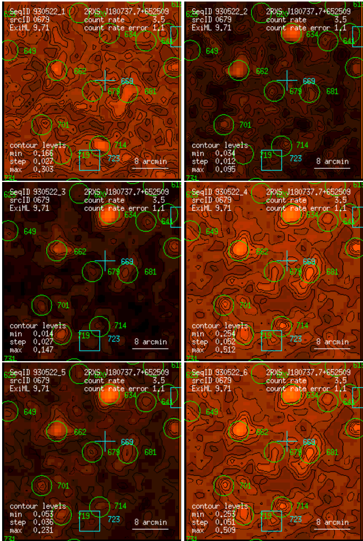
Figure 679: RASS 930522: detection 0679: band rate images, Gaussian filter: (1) PSPC channels 11 – 41, (2) 52 – 90, (3) 91 – 201, (4) 11 – 235, (5) 52 – 201, (6) 11 – 201. Broad band rates in counts/ks. Band rate contour levels in counts/ks/arcmin 2 .
