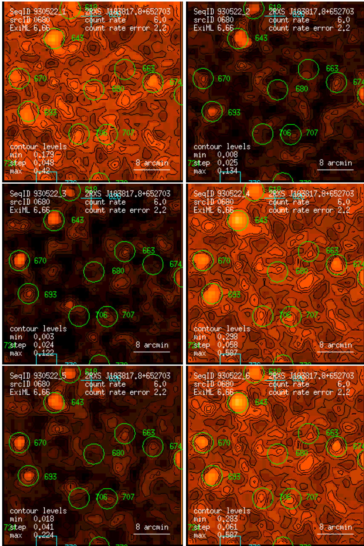
Figure 680: RASS 930522: detection 0680: band rate images, Gaussian filter: (1) PSPC channels 11 – 41, (2) 52 – 90, (3) 91 – 201, (4) 11 – 235, (5) 52 – 201, (6) 11 – 201. Broad band rates in counts/ks. Band rate contour levels in counts/ks/arcmin 2 .
