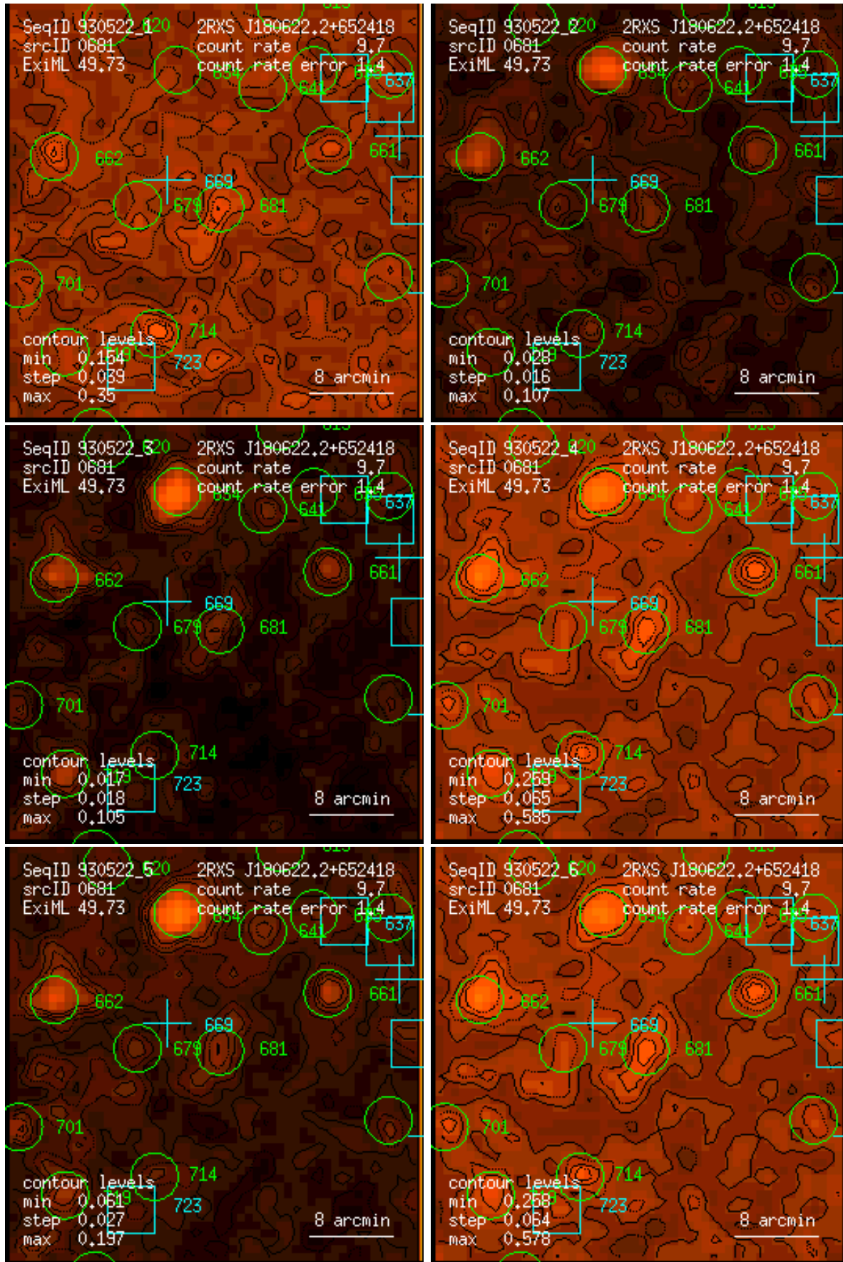
Figure 681: RASS 930522: detection 0681: band rate images, Gaussian filter: (1) PSPC channels 11 – 41, (2) 52 – 90, (3) 91 – 201, (4) 11 – 235, (5) 52 – 201, (6) 11 – 201. Broad band rates in counts/ks. Band rate contour levels in counts/ks/arcmin 2 .
