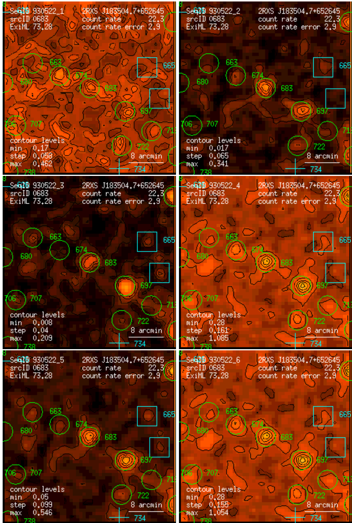
Figure 683: RASS 930522: detection 0683: band rate images, Gaussian filter: (1) PSPC channels 11 – 41, (2) 52 – 90, (3) 91 – 201, (4) 11 – 235, (5) 52 – 201, (6) 11 – 201. Broad band rates in counts/ks. Band rate contour levels in counts/ks/arcmin 2 .
