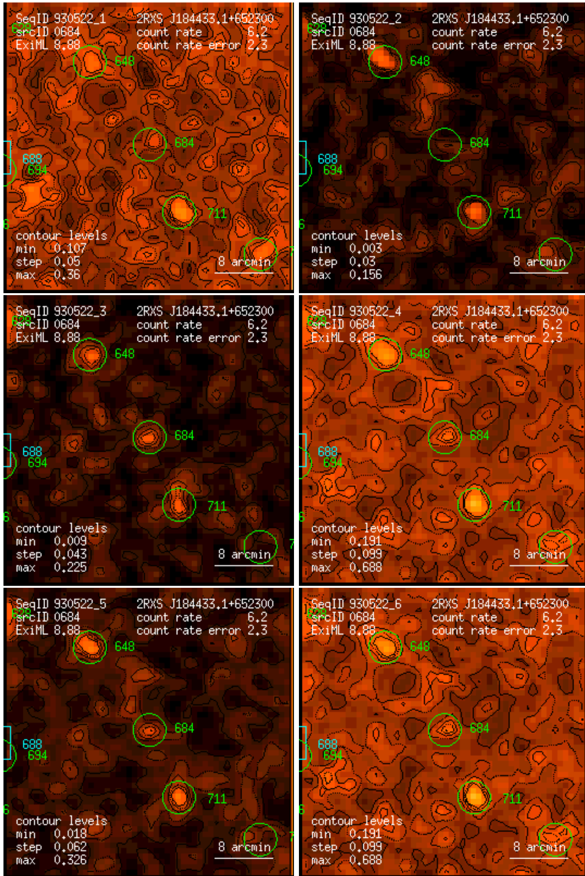
Figure 684: RASS 930522: detection 0684: band rate images, Gaussian filter: (1) PSPC channels 11 – 41, (2) 52 – 90, (3) 91 – 201, (4) 11 – 235, (5) 52 – 201, (6) 11 – 201. Broad band rates in counts/ks. Band rate contour levels in counts/ks/arcmin 2 .
