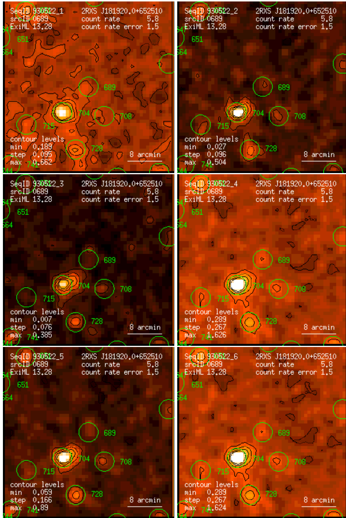
Figure 689: RASS 930522: detection 0689: band rate images, Gaussian filter: (1) PSPC channels 11 – 41, (2) 52 – 90, (3) 91 – 201, (4) 11 – 235, (5) 52 – 201, (6) 11 – 201. Broad band rates in counts/ks. Band rate contour levels in counts/ks/arcmin 2 .
