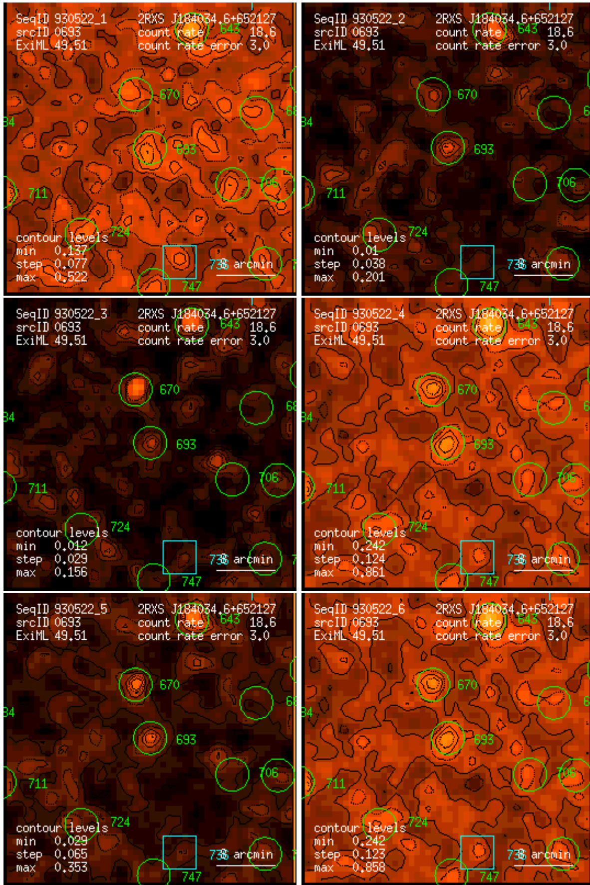
Figure 693: RASS 930522: detection 0693: band rate images, Gaussian filter: (1) PSPC channels 11 – 41, (2) 52 – 90, (3) 91 – 201, (4) 11 – 235, (5) 52 – 201, (6) 11 – 201. Broad band rates in counts/ks. Band rate contour levels in counts/ks/arcmin 2 .
