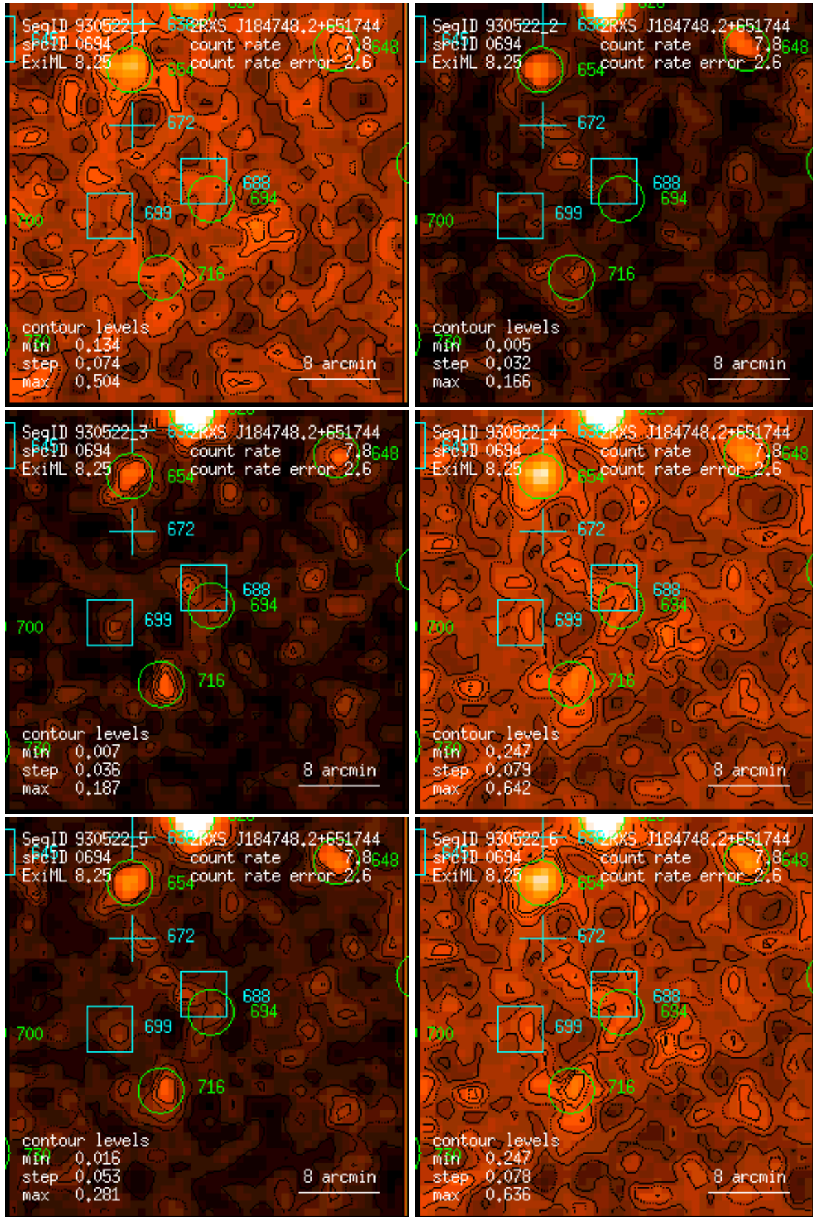
Figure 694: RASS 930522: detection 0694: band rate images, Gaussian filter: (1) PSPC channels 11 – 41, (2) 52 – 90, (3) 91 – 201, (4) 11 – 235, (5) 52 – 201, (6) 11 – 201. Broad band rates in counts/ks. Band rate contour levels in counts/ks/arcmin 2 .
