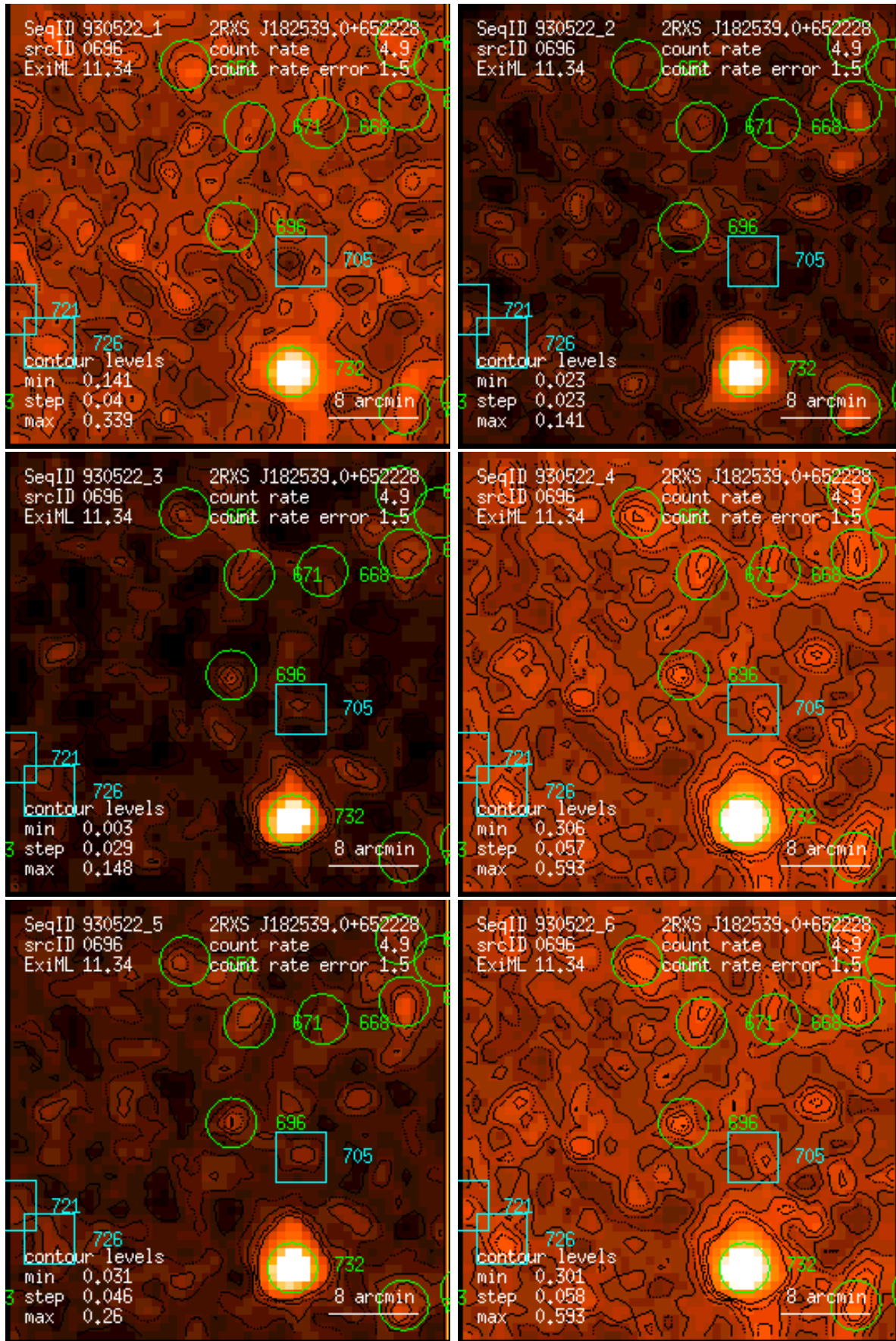
Figure 696: RASS 930522: detection 0696: band rate images, Gaussian filter: (1) PSPC channels 11 – 41, (2) 52 – 90, (3) 91 – 201, (4) 11 – 235, (5) 52 – 201, (6) 11 – 201. Broad band rates in counts/ks. Band rate contour levels in counts/ks/arcmin 2 .
