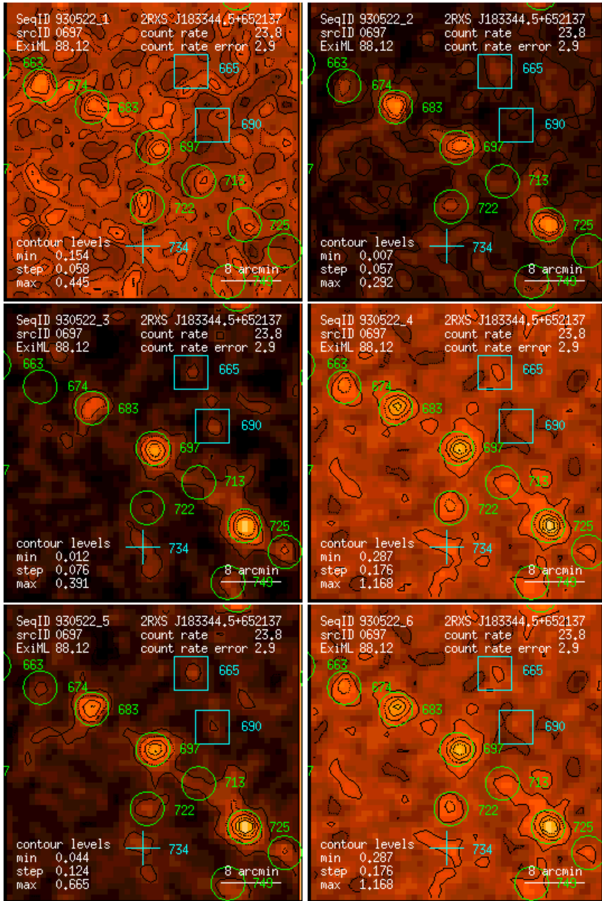
Figure 697: RASS 930522: detection 0697: band rate images, Gaussian filter: (1) PSPC channels 11 – 41, (2) 52 – 90, (3) 91 – 201, (4) 11 – 235, (5) 52 – 201, (6) 11 – 201. Broad band rates in counts/ks. Band rate contour levels in counts/ks/arcmin 2 .
