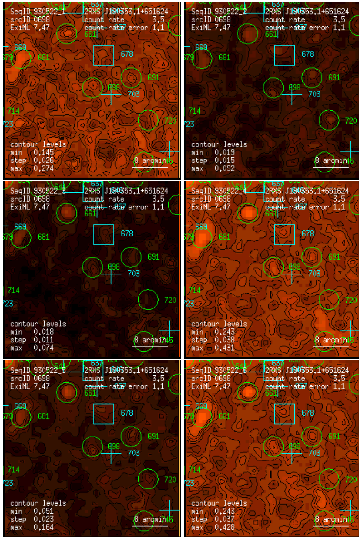
Figure 698: RASS 930522: detection 0698: band rate images, Gaussian filter: (1) PSPC channels 11 – 41, (2) 52 – 90, (3) 91 – 201, (4) 11 – 235, (5) 52 – 201, (6) 11 – 201. Broad band rates in counts/ks. Band rate contour levels in counts/ks/arcmin 2 .
