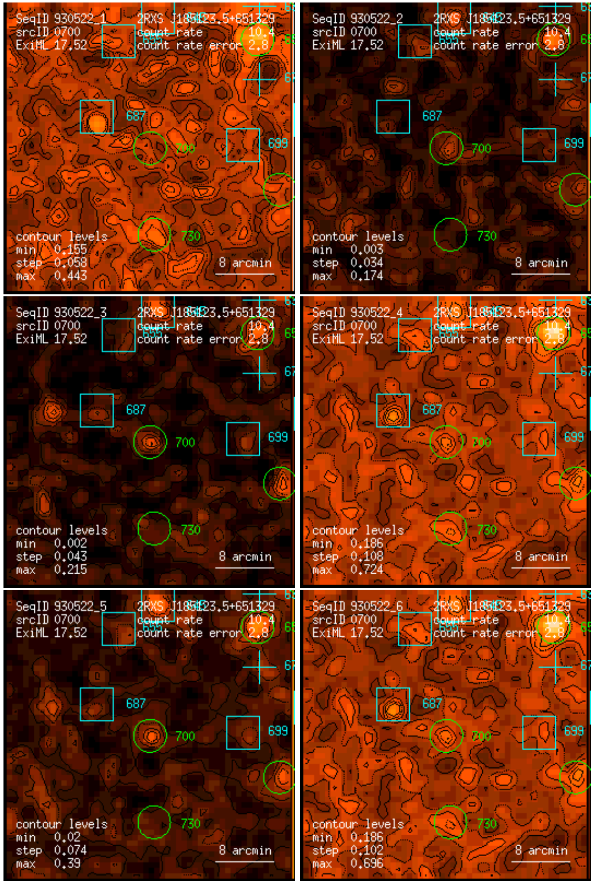
Figure 700: RASS 930522: detection 0700: band rate images, Gaussian filter: (1) PSPC channels 11 – 41, (2) 52 – 90, (3) 91 – 201, (4) 11 – 235, (5) 52 – 201, (6) 11 – 201. Broad band rates in counts/ks. Band rate contour levels in counts/ks/arcmin 2 .
