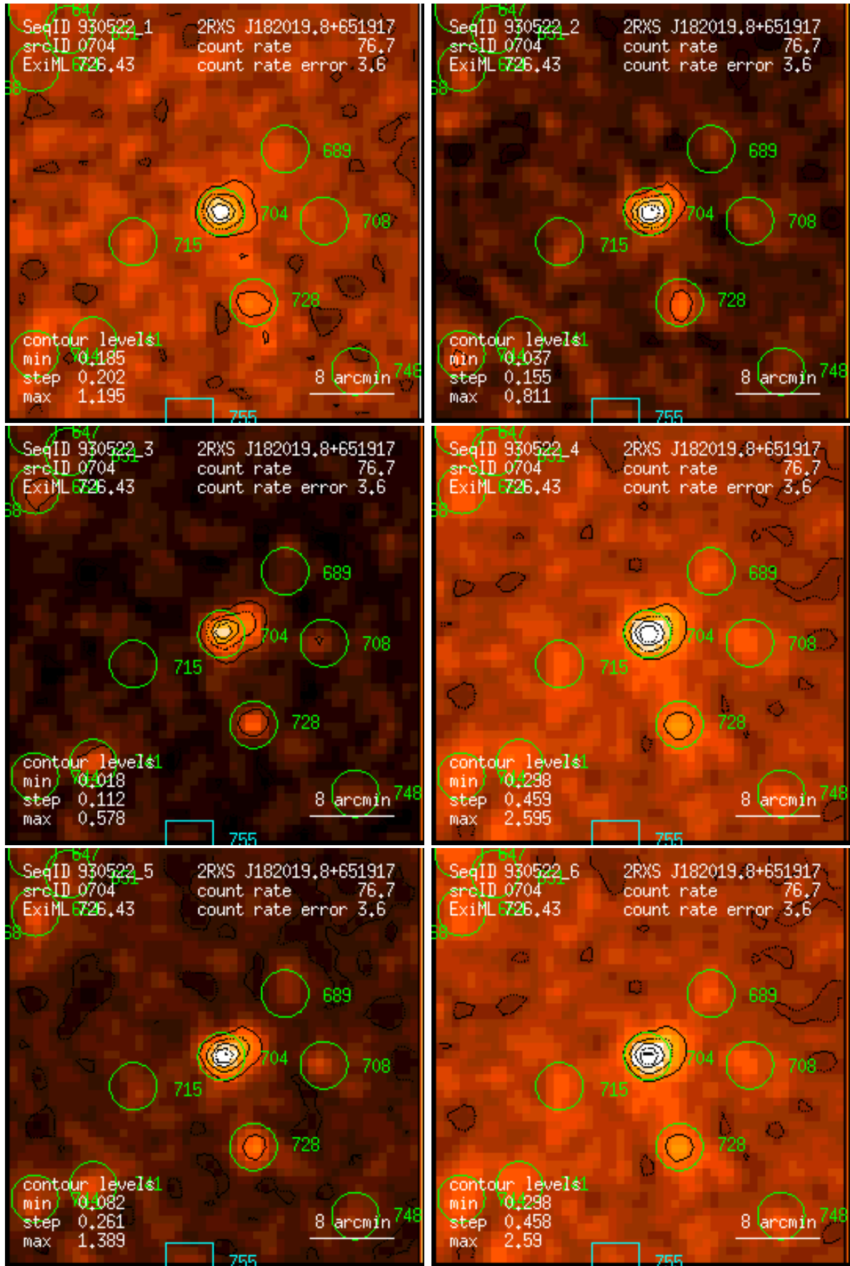
Figure 704: RASS 930522: detection 0704: band rate images, Gaussian filter: (1) PSPC channels 11 – 41, (2) 52 – 90, (3) 91 – 201, (4) 11 – 235, (5) 52 – 201, (6) 11 – 201. Broad band rates in counts/ks. Band rate contour levels in counts/ks/arcmin 2 .
