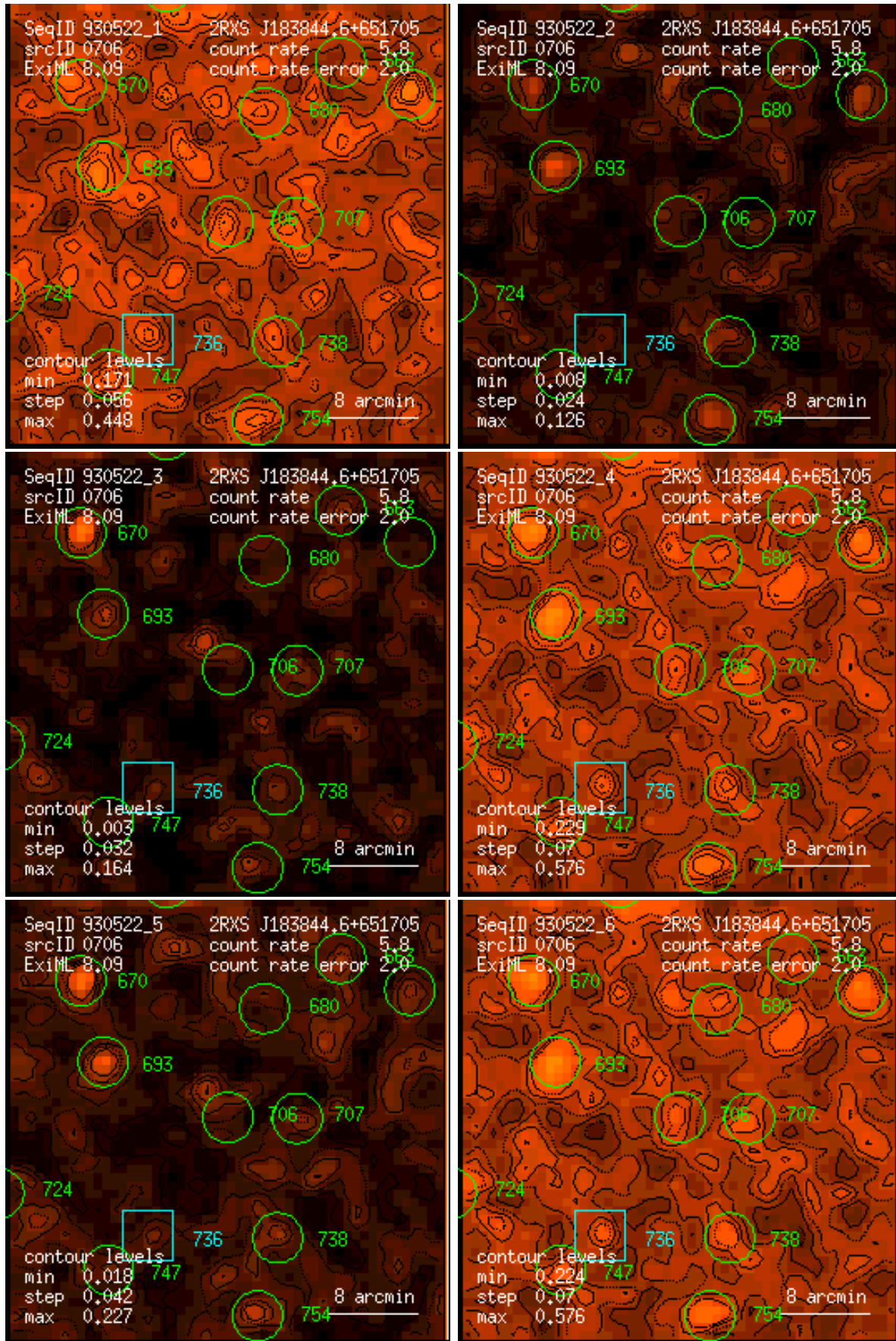
Figure 706: RASS 930522: detection 0706: band rate images, Gaussian filter: (1) PSPC channels 11 – 41, (2) 52 – 90, (3) 91 – 201, (4) 11 – 235, (5) 52 – 201, (6) 11 – 201. Broad band rates in counts/ks. Band rate contour levels in counts/ks/arcmin 2 .
