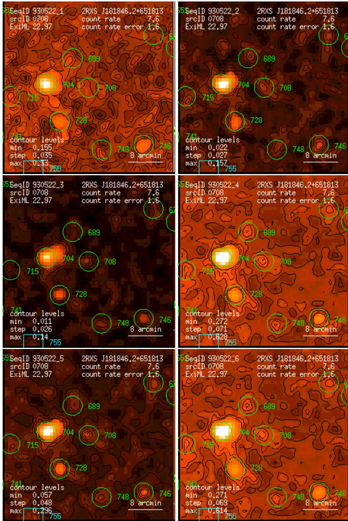
Figure 708: RASS 930522: detection 0708: band rate images, Gaussian filter: (1) PSPC channels 11 – 41, (2) 52 – 90, (3) 91 – 201, (4) 11 – 235, (5) 52 – 201, (6) 11 – 201. Broad band rates in counts/ks. Band rate contour levels in counts/ks/arcmin 2 .
