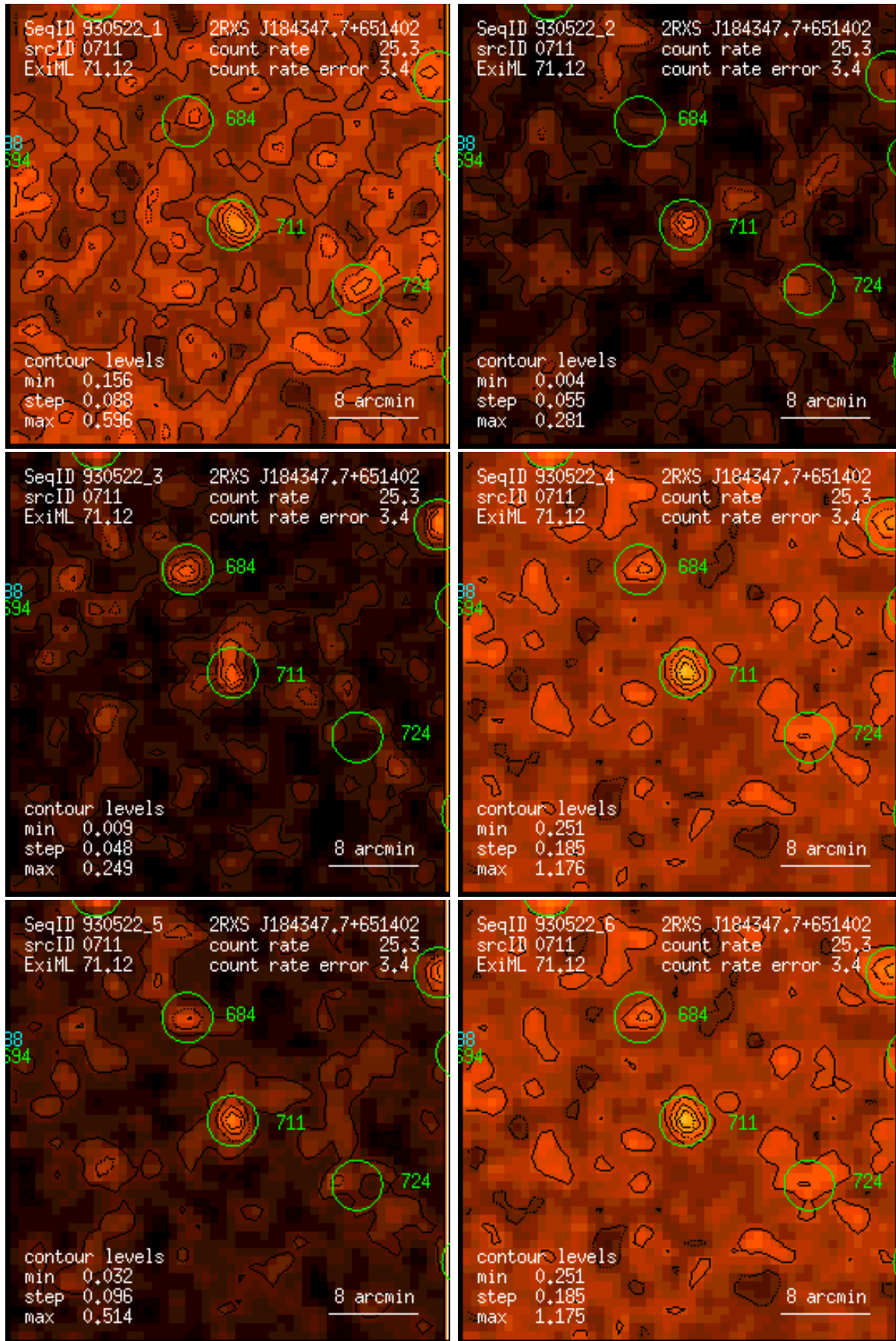
Figure 711: RASS 930522: detection 0711: band rate images, Gaussian filter: (1) PSPC channels 11 – 41, (2) 52 – 90, (3) 91 – 201, (4) 11 – 235, (5) 52 – 201, (6) 11 – 201. Broad band rates in counts/ks. Band rate contour levels in counts/ks/arcmin 2 .
