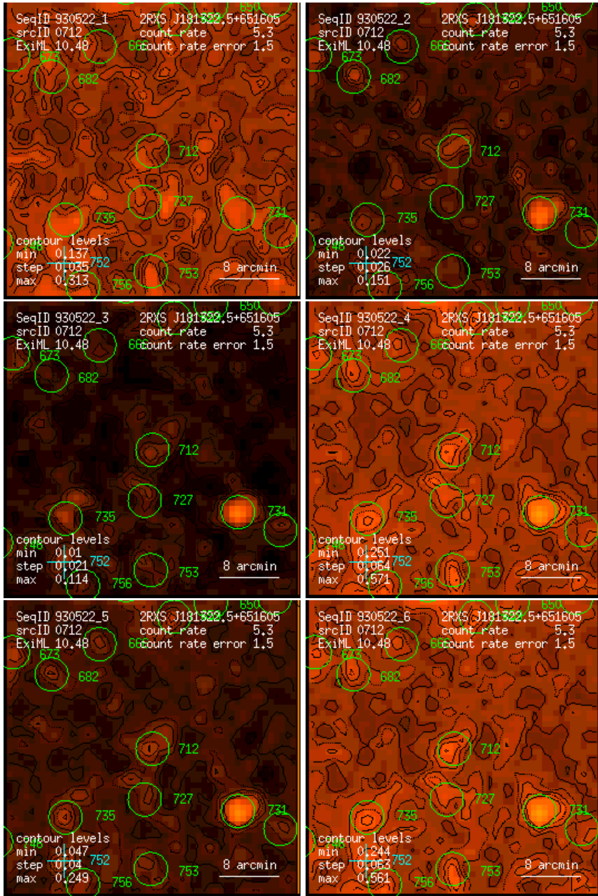
Figure 712: RASS 930522: detection 0712: band rate images, Gaussian filter: (1) PSPC channels 11 – 41, (2) 52 – 90, (3) 91 – 201, (4) 11 – 235, (5) 52 – 201, (6) 11 – 201. Broad band rates in counts/ks. Band rate contour levels in counts/ks/arcmin 2 .
