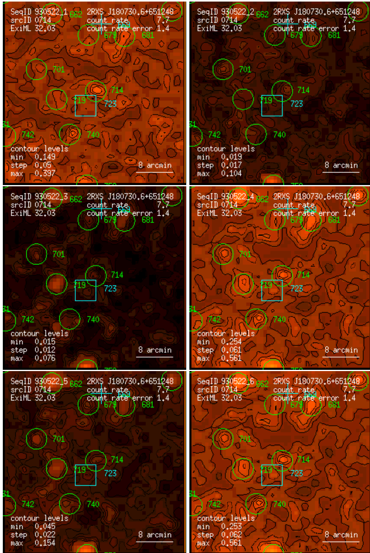
Figure 714: RASS 930522: detection 0714: band rate images, Gaussian filter: (1) PSPC channels 11 – 41, (2) 52 – 90, (3) 91 – 201, (4) 11 – 235, (5) 52 – 201, (6) 11 – 201. Broad band rates in counts/ks. Band rate contour levels in counts/ks/arcmin 2 .
