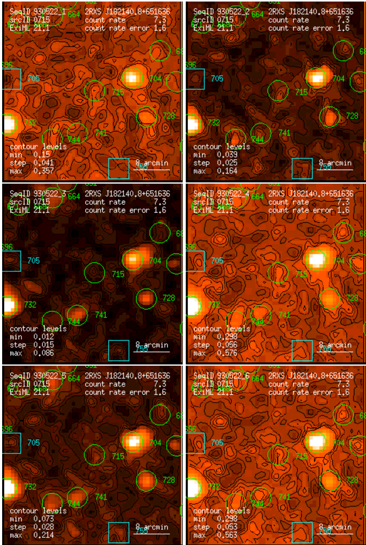
Figure 715: RASS 930522: detection 0715: band rate images, Gaussian filter: (1) PSPC channels 11 – 41, (2) 52 – 90, (3) 91 – 201, (4) 11 – 235, (5) 52 – 201, (6) 11 – 201. Broad band rates in counts/ks. Band rate contour levels in counts/ks/arcmin 2 .
