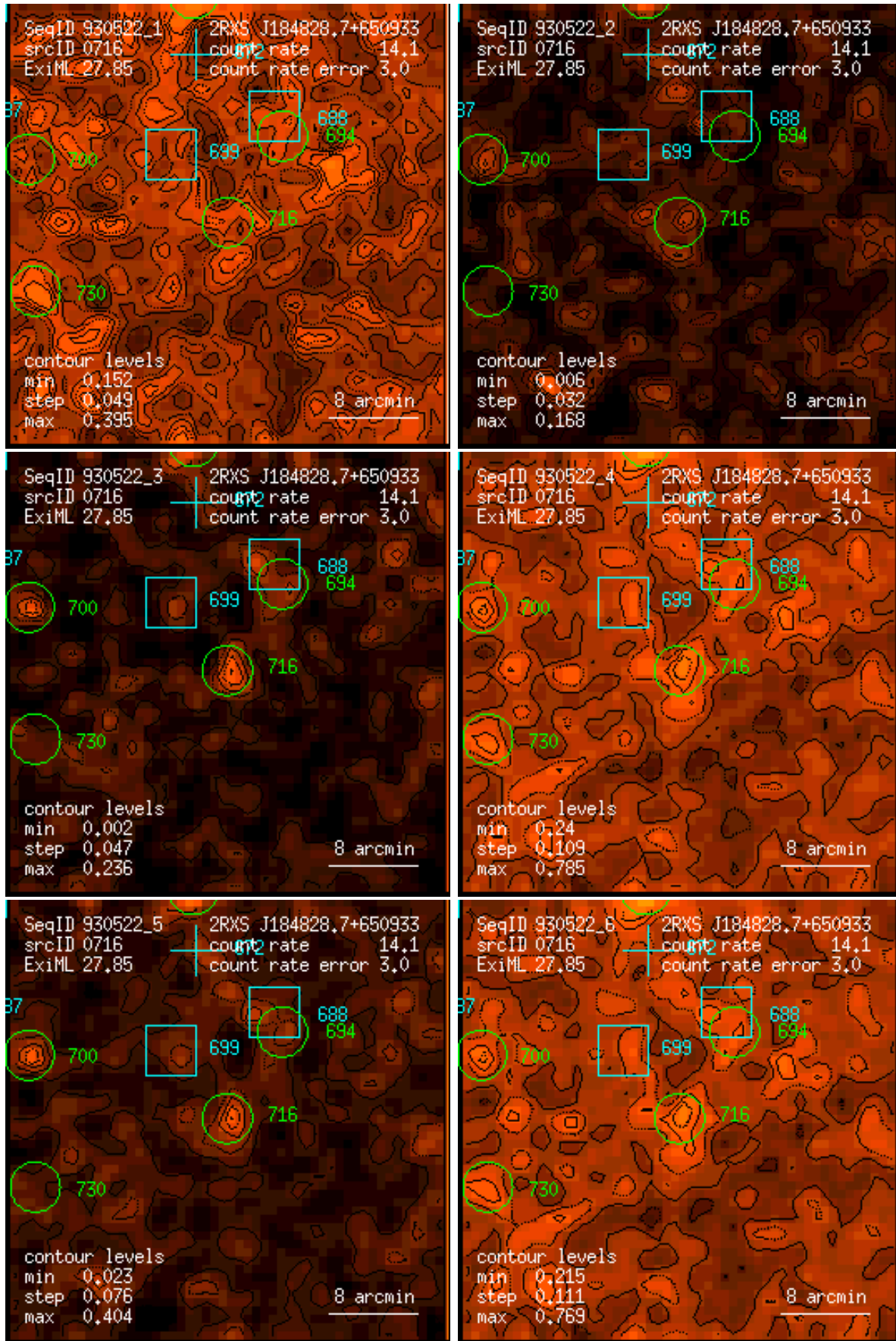
Figure 716: RASS 930522: detection 0716: band rate images, Gaussian filter: (1) PSPC channels 11 – 41, (2) 52 – 90, (3) 91 – 201, (4) 11 – 235, (5) 52 – 201, (6) 11 – 201. Broad band rates in counts/ks. Band rate contour levels in counts/ks/arcmin 2 .
