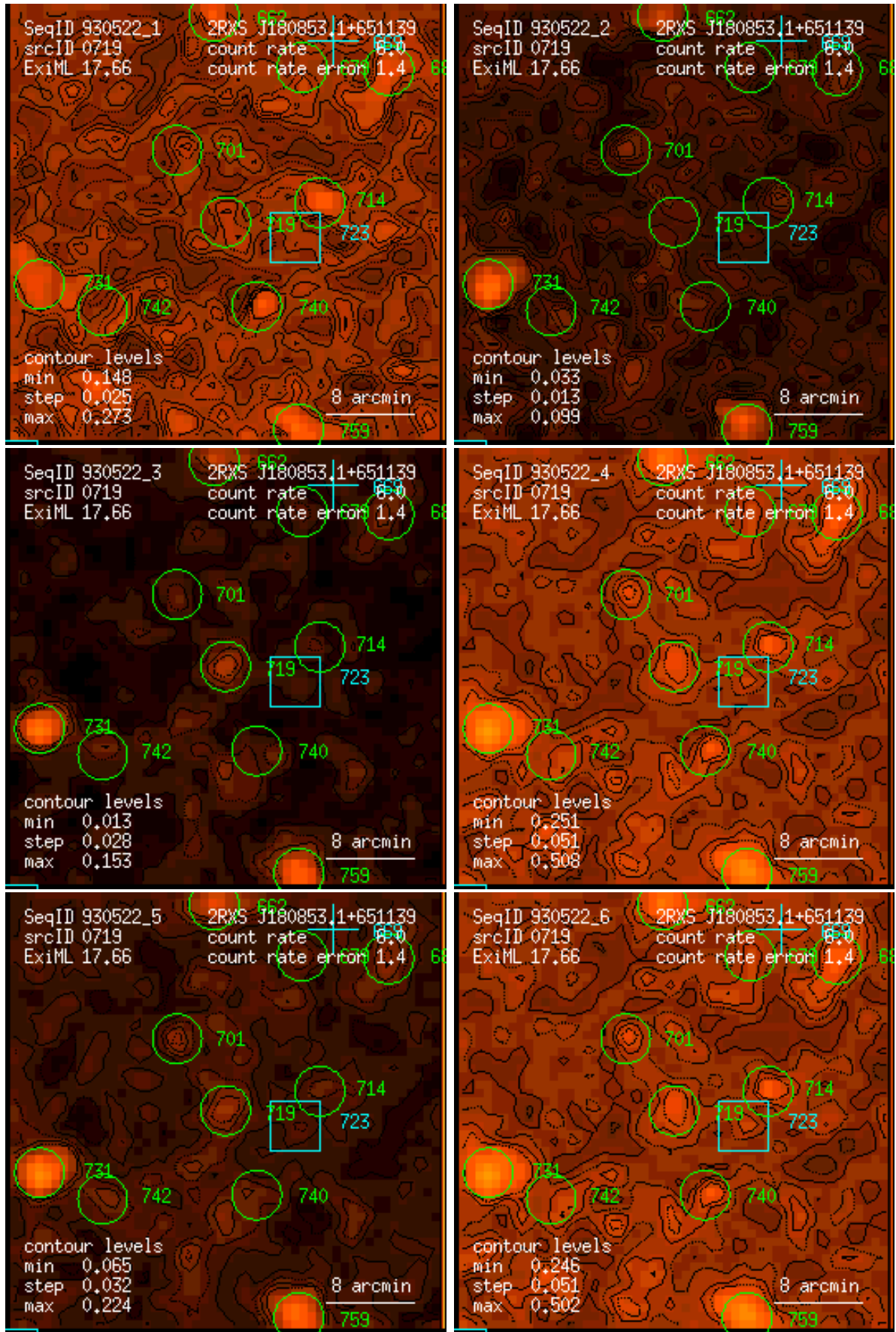
Figure 719: RASS 930522: detection 0719: band rate images, Gaussian filter: (1) PSPC channels 11 – 41, (2) 52 – 90, (3) 91 – 201, (4) 11 – 235, (5) 52 – 201, (6) 11 – 201. Broad band rates in counts/ks. Band rate contour levels in counts/ks/arcmin 2 .
