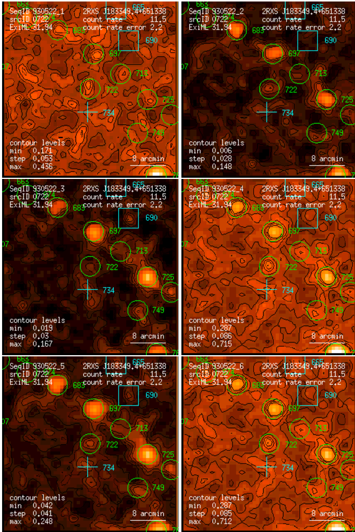
Figure 722: RASS 930522: detection 0722: band rate images, Gaussian filter: (1) PSPC channels 11 – 41, (2) 52 – 90, (3) 91 – 201, (4) 11 – 235, (5) 52 – 201, (6) 11 – 201. Broad band rates in counts/ks. Band rate contour levels in counts/ks/arcmin 2 .
