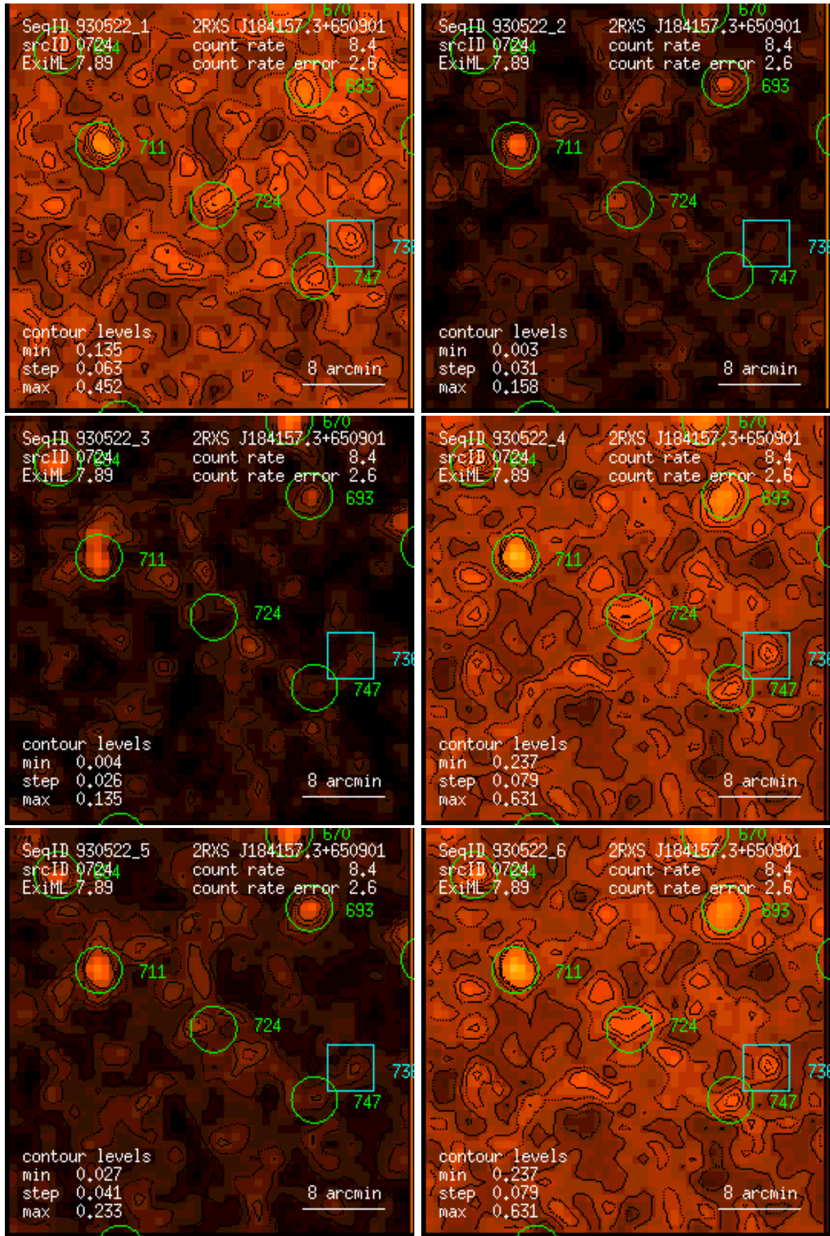
Figure 724: RASS 930522: detection 0724: band rate images, Gaussian filter: (1) PSPC channels 11 – 41, (2) 52 – 90, (3) 91 – 201, (4) 11 – 235, (5) 52 – 201, (6) 11 – 201. Broad band rates in counts/ks. Band rate contour levels in counts/ks/arcmin 2 .
