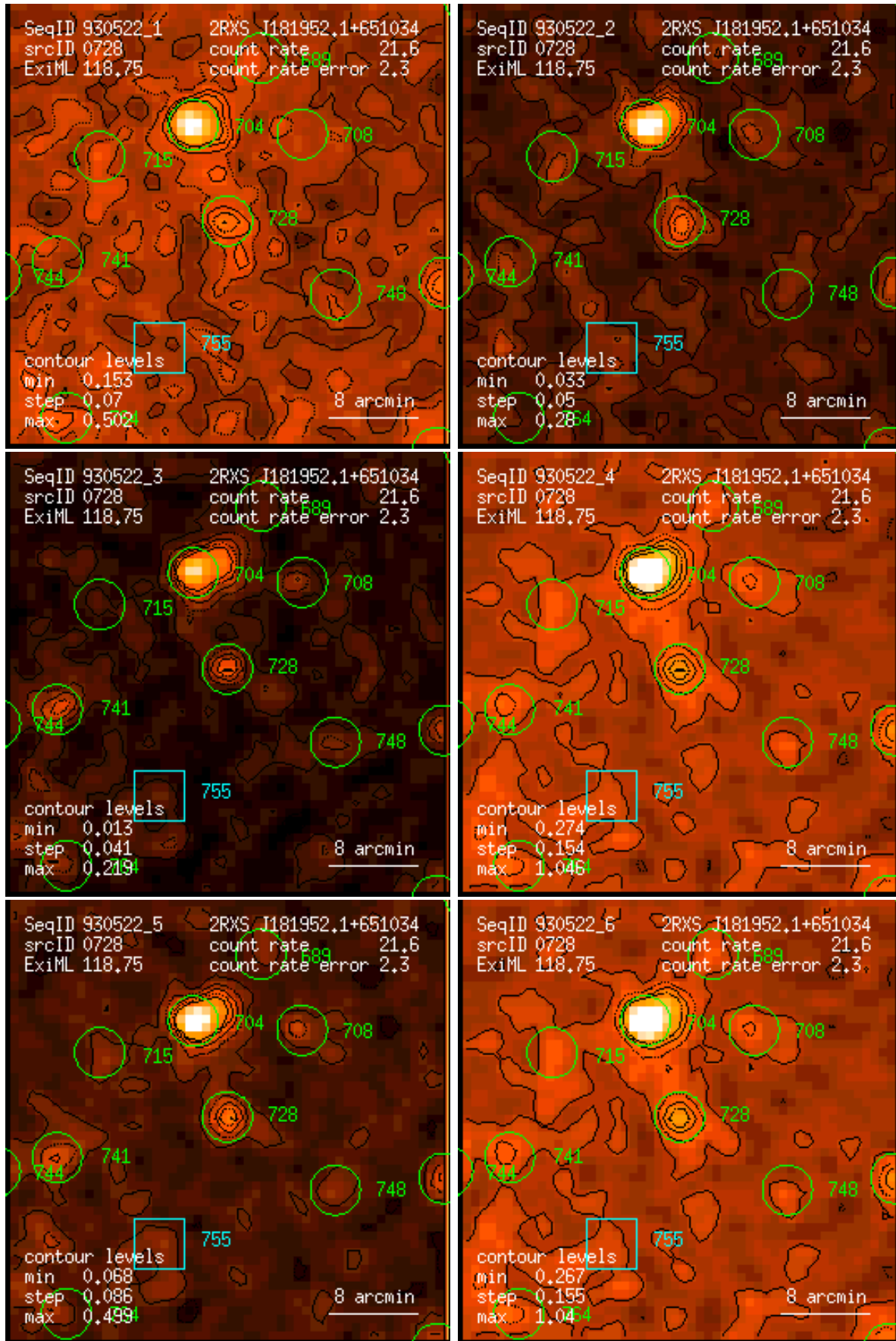
Figure 728: RASS 930522: detection 0728: band rate images, Gaussian filter: (1) PSPC channels 11 – 41, (2) 52 – 90, (3) 91 – 201, (4) 11 – 235, (5) 52 – 201, (6) 11 – 201. Broad band rates in counts/ks. Band rate contour levels in counts/ks/arcmin 2 .
