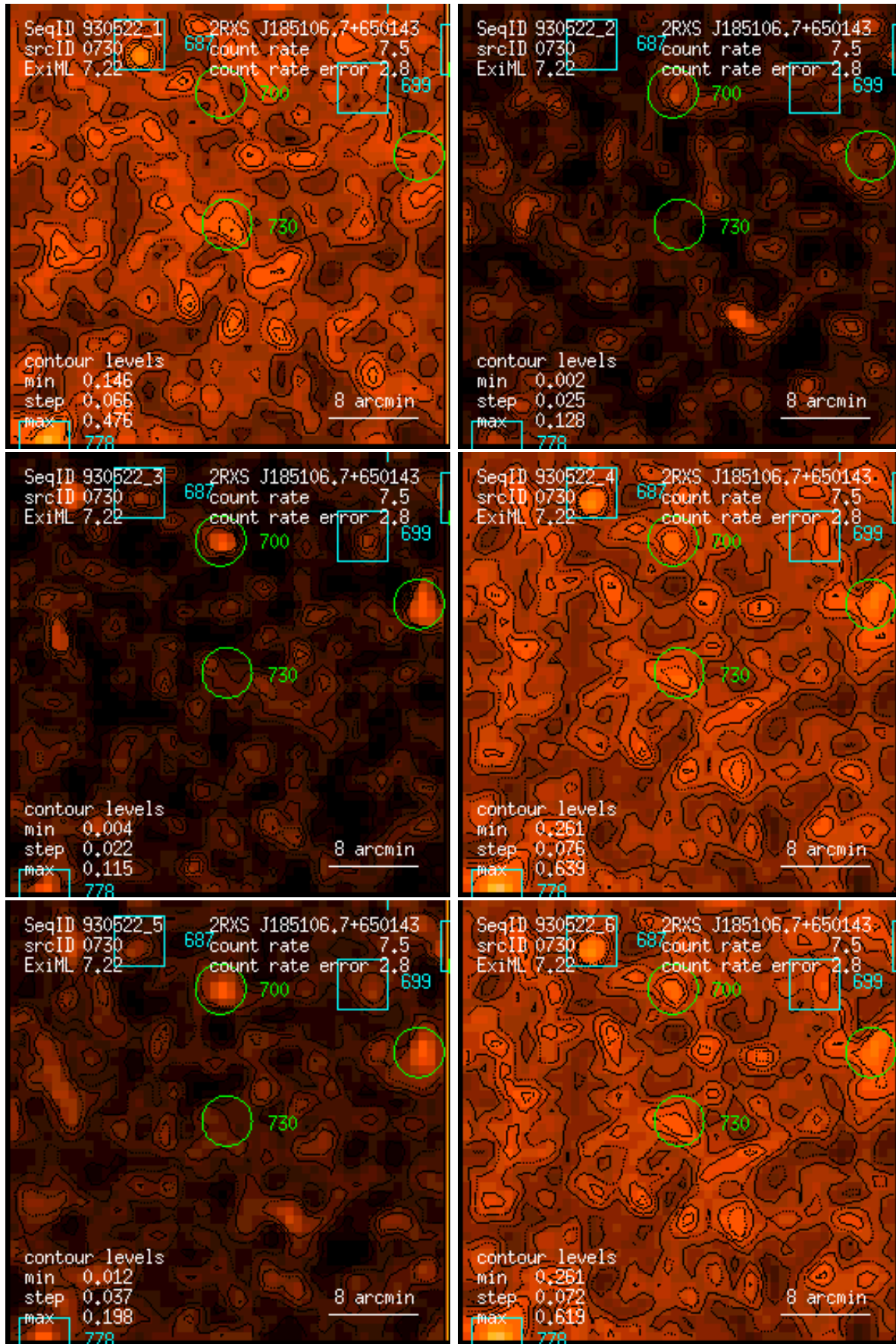
Figure 730: RASS 930522: detection 0730: band rate images, Gaussian filter: (1) PSPC channels 11 – 41, (2) 52 – 90, (3) 91 – 201, (4) 11 – 235, (5) 52 – 201, (6) 11 – 201. Broad band rates in counts/ks. Band rate contour levels in counts/ks/arcmin 2 .
