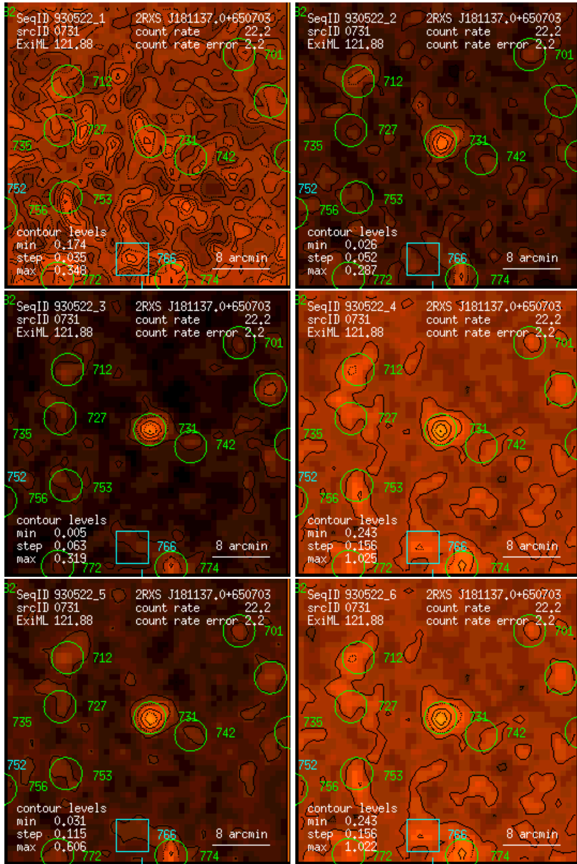
Figure 731: RASS 930522: detection 0731: band rate images, Gaussian filter: (1) PSPC channels 11 – 41, (2) 52 – 90, (3) 91 – 201, (4) 11 – 235, (5) 52 – 201, (6) 11 – 201. Broad band rates in counts/ks. Band rate contour levels in counts/ks/arcmin 2 .
