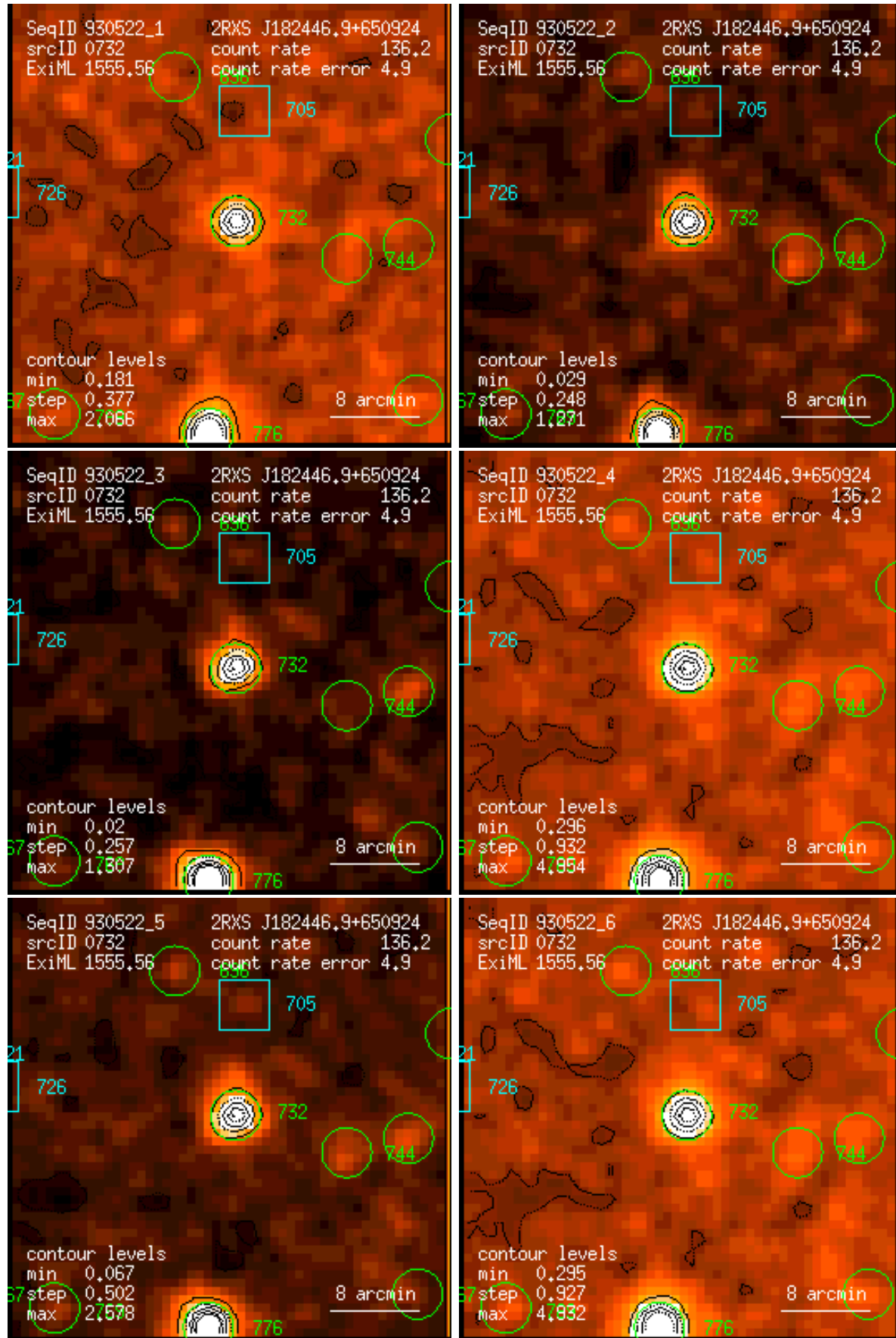
Figure 732: RASS 930522: detection 0732: band rate images, Gaussian filter: (1) PSPC channels 11 – 41, (2) 52 – 90, (3) 91 – 201, (4) 11 – 235, (5) 52 – 201, (6) 11 – 201. Broad band rates in counts/ks. Band rate contour levels in counts/ks/arcmin 2 .
