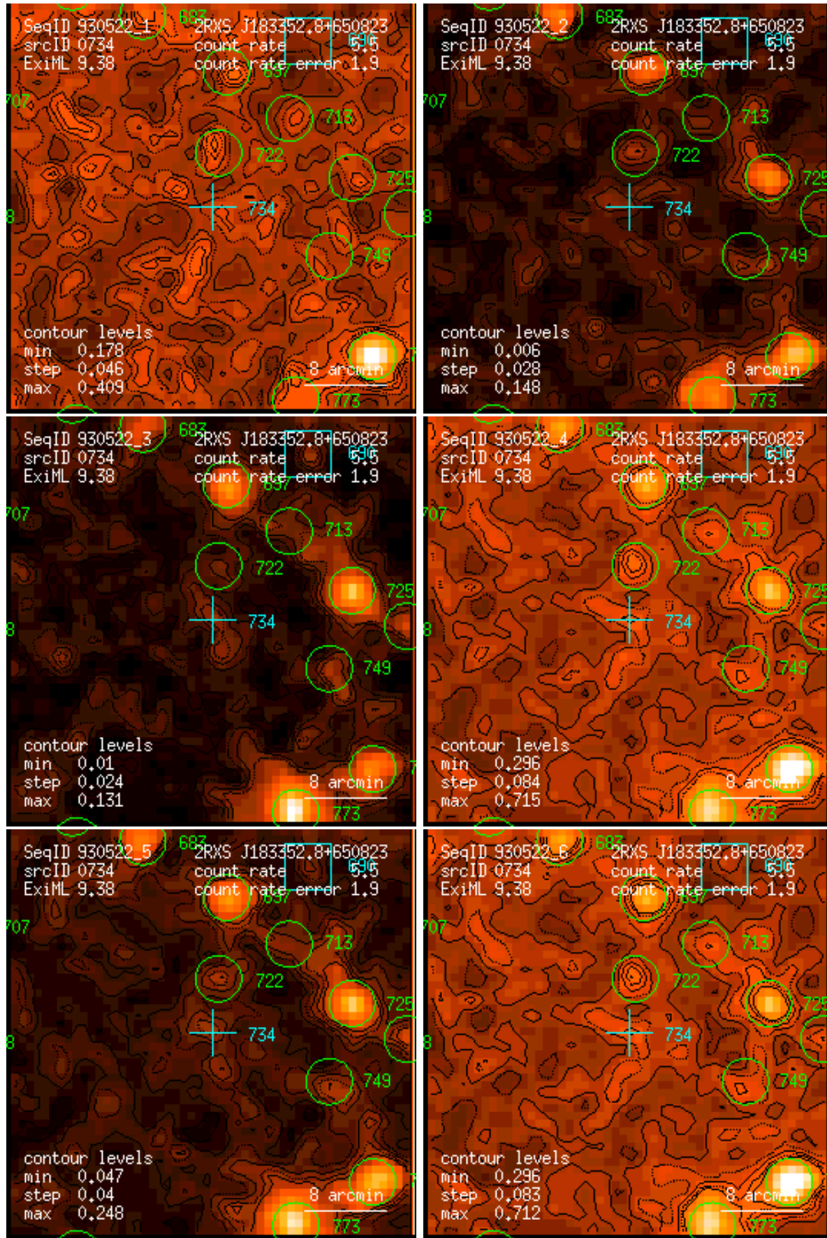
Figure 734: RASS 930522: detection 0734: band rate images, Gaussian filter: (1) PSPC channels 11 – 41, (2) 52 – 90, (3) 91 – 201, (4) 11 – 235, (5) 52 – 201, (6) 11 – 201. Broad band rates in counts/ks. Band rate contour levels in counts/ks/arcmin 2 .
