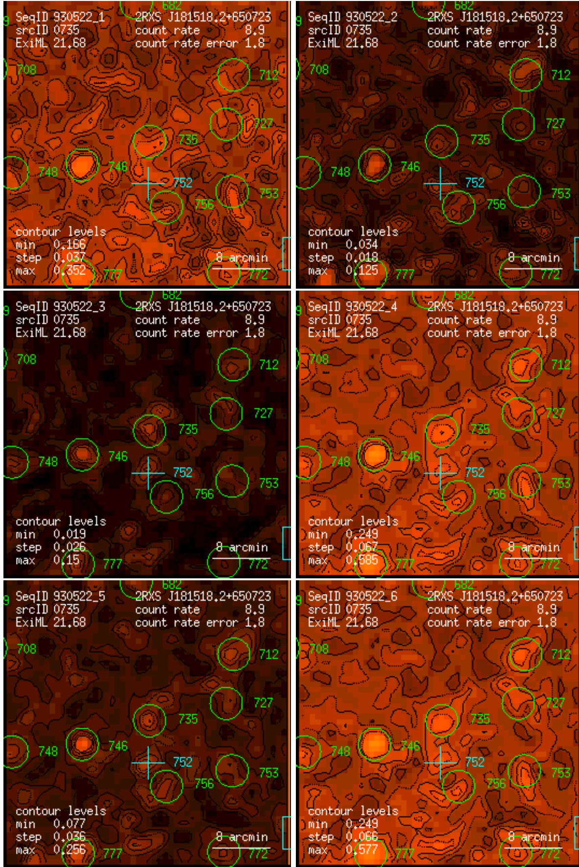
Figure 735: RASS 930522: detection 0735: band rate images, Gaussian filter: (1) PSPC channels 11 – 41, (2) 52 – 90, (3) 91 – 201, (4) 11 – 235, (5) 52 – 201, (6) 11 – 201. Broad band rates in counts/ks. Band rate contour levels in counts/ks/arcmin 2 .
