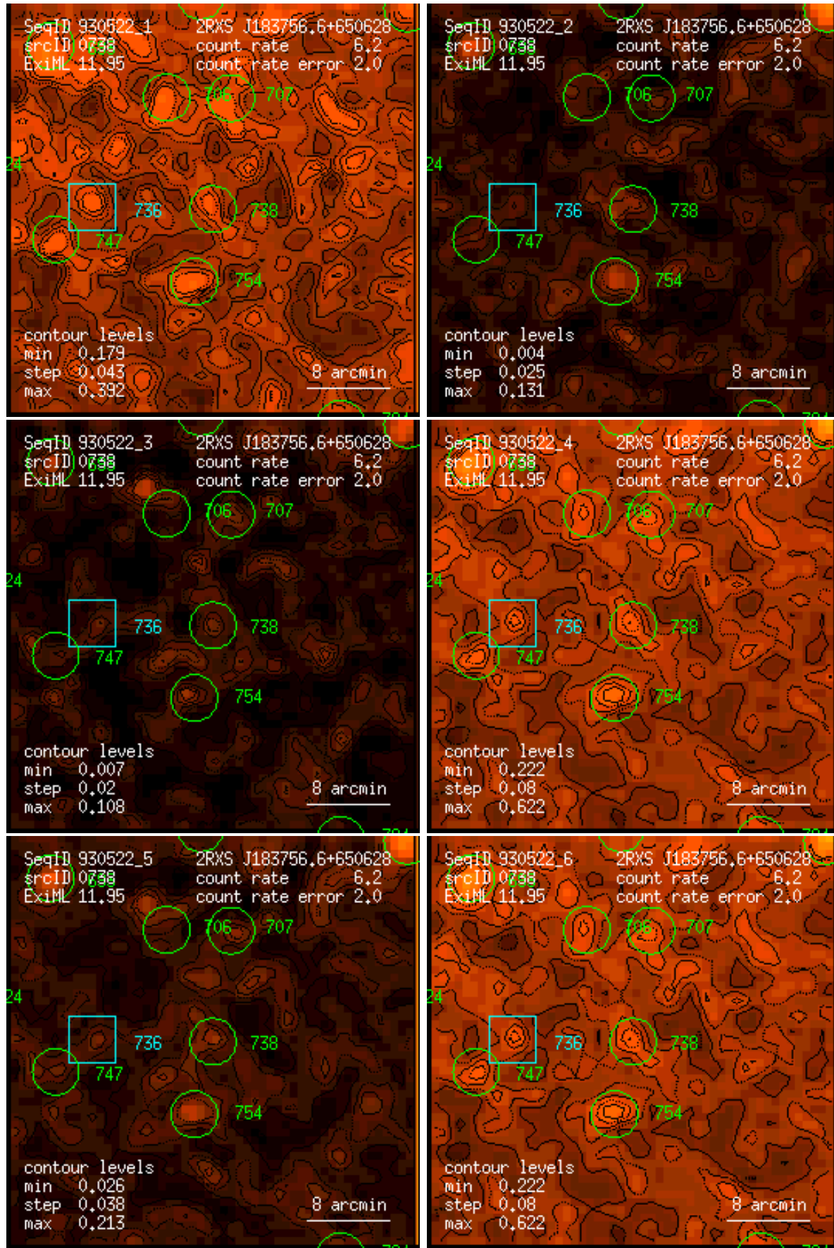
Figure 738: RASS 930522: detection 0738: band rate images, Gaussian filter: (1) PSPC channels 11 – 41, (2) 52 – 90, (3) 91 – 201, (4) 11 – 235, (5) 52 – 201, (6) 11 – 201. Broad band rates in counts/ks. Band rate contour levels in counts/ks/arcmin 2 .
