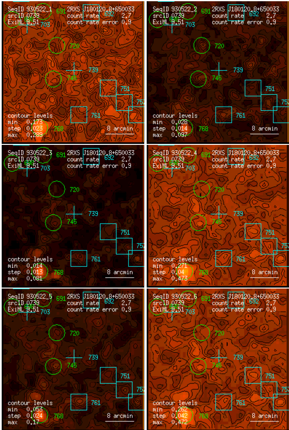
Figure 739: RASS 930522: detection 0739: band rate images, Gaussian filter: (1) PSPC channels 11 – 41, (2) 52 – 90, (3) 91 – 201, (4) 11 – 235, (5) 52 – 201, (6) 11 – 201. Broad band rates in counts/ks. Band rate contour levels in counts/ks/arcmin 2 .
