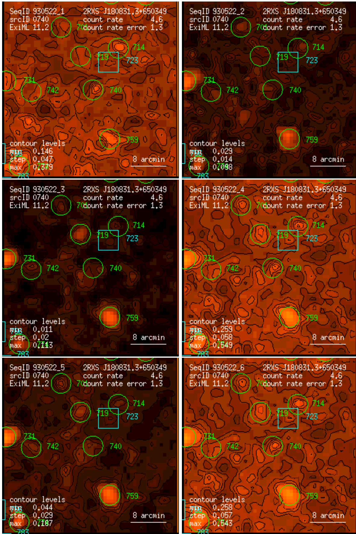
Figure 740: RASS 930522: detection 0740: band rate images, Gaussian filter: (1) PSPC channels 11 – 41, (2) 52 – 90, (3) 91 – 201, (4) 11 – 235, (5) 52 – 201, (6) 11 – 201. Broad band rates in counts/ks. Band rate contour levels in counts/ks/arcmin 2 .
