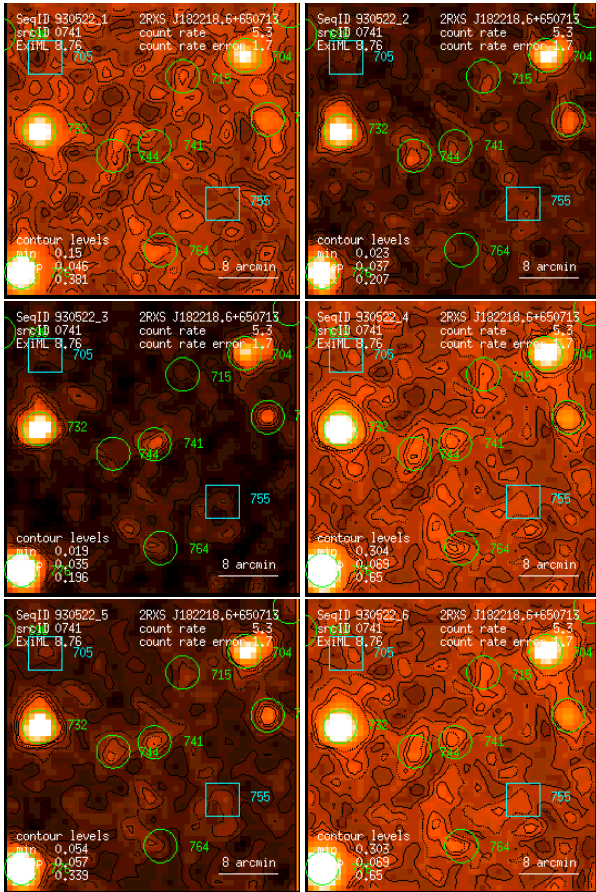
Figure 741: RASS 930522: detection 0741: band rate images, Gaussian filter: (1) PSPC channels 11 – 41, (2) 52 – 90, (3) 91 – 201, (4) 11 – 235, (5) 52 – 201, (6) 11 – 201. Broad band rates in counts/ks. Band rate contour levels in counts/ks/arcmin 2 .
