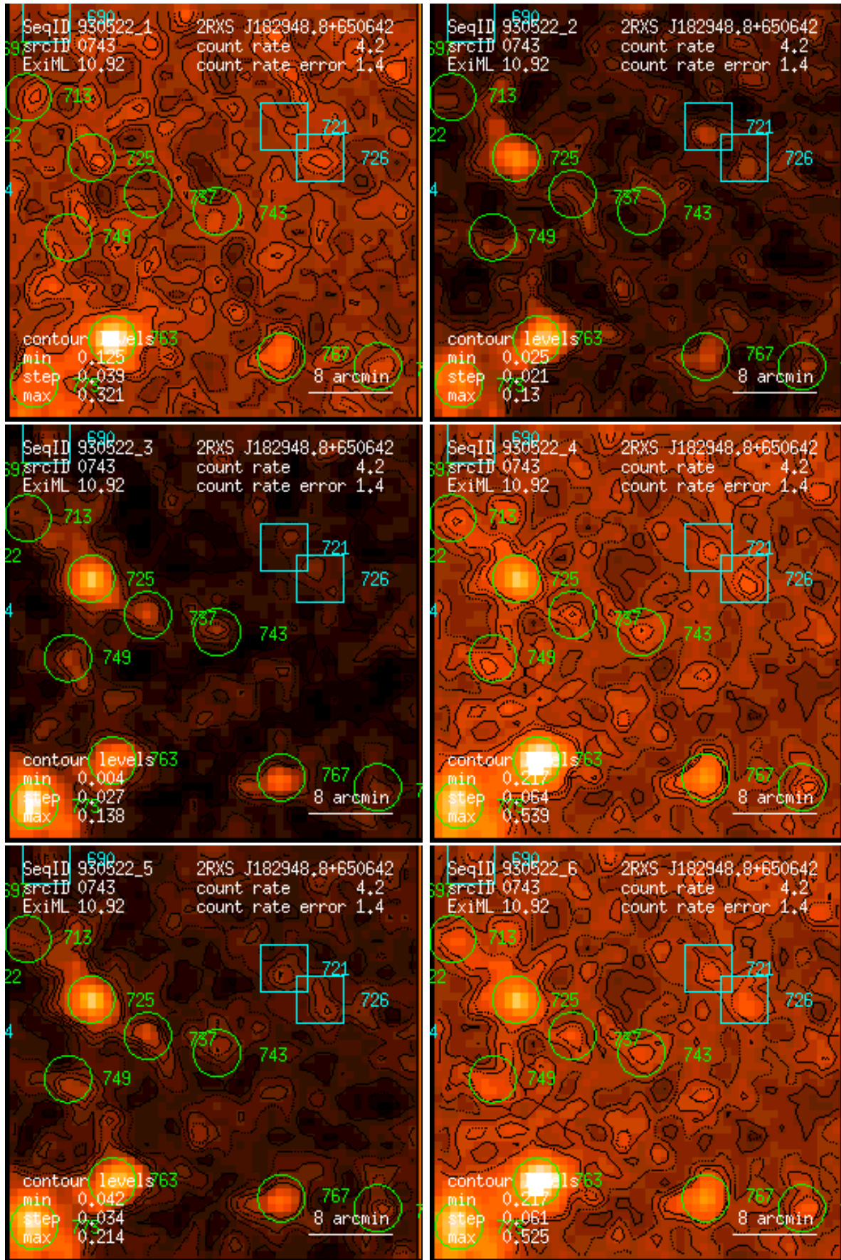
Figure 743: RASS 930522: detection 0743: band rate images, Gaussian filter: (1) PSPC channels 11 – 41, (2) 52 – 90, (3) 91 – 201, (4) 11 – 235, (5) 52 – 201, (6) 11 – 201. Broad band rates in counts/ks. Band rate contour levels in counts/ks/arcmin 2 .
