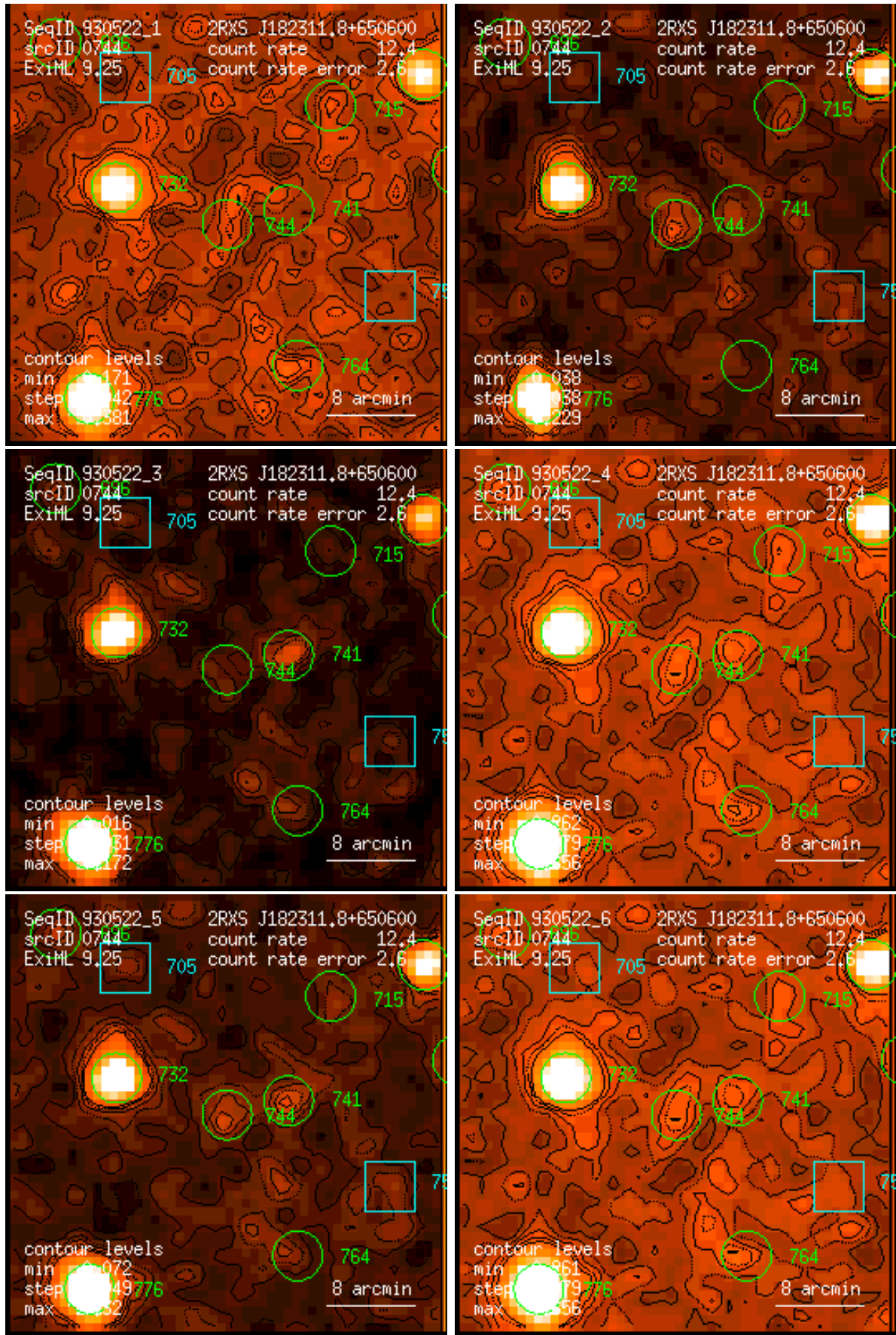
Figure 744: RASS 930522: detection 0744: band rate images, Gaussian filter: (1) PSPC channels 11 – 41, (2) 52 – 90, (3) 91 – 201, (4) 11 – 235, (5) 52 – 201, (6) 11 – 201. Broad band rates in counts/ks. Band rate contour levels in counts/ks/arcmin 2 .
